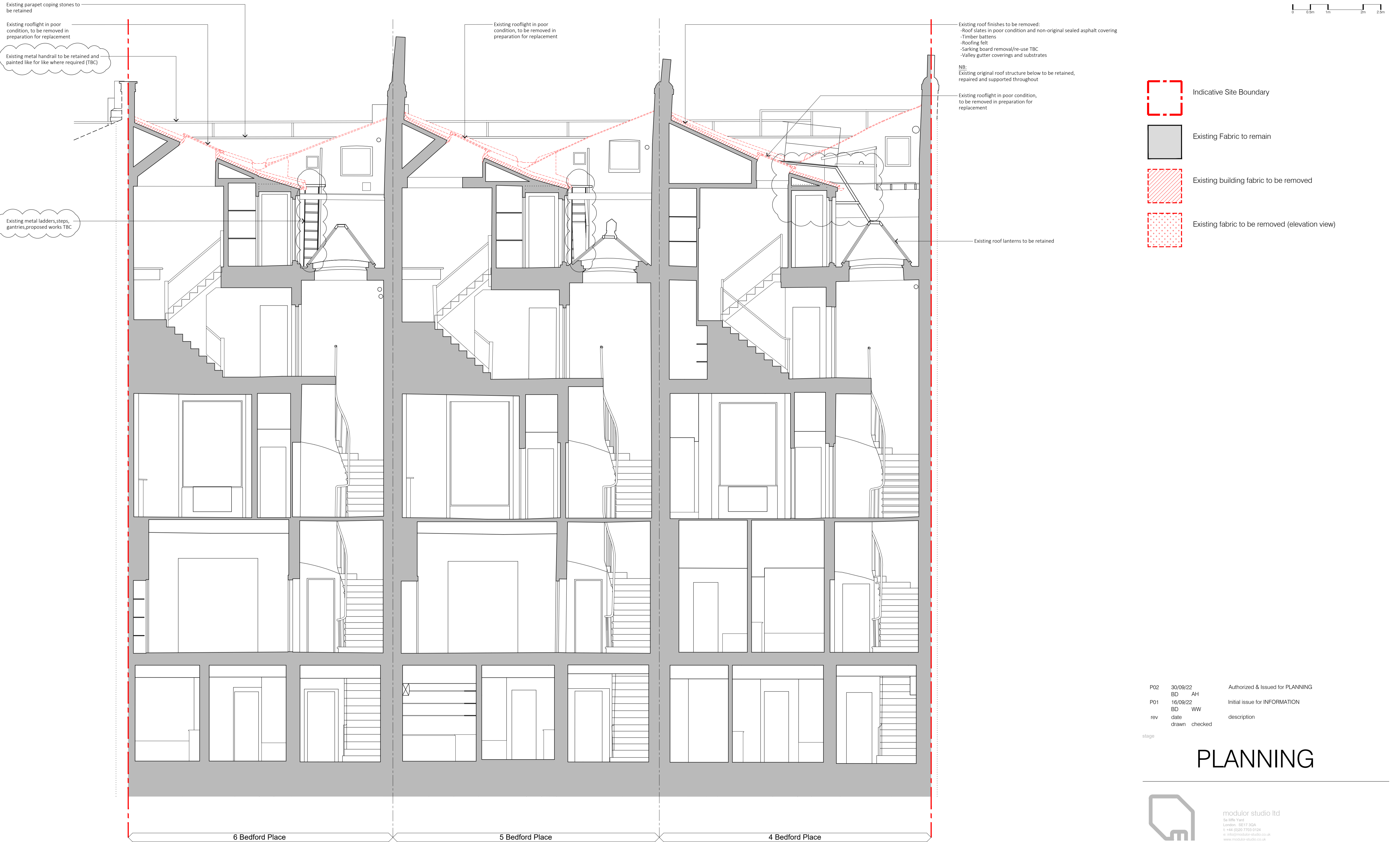
1 Demolition Section B-B 1:50 @ A1
