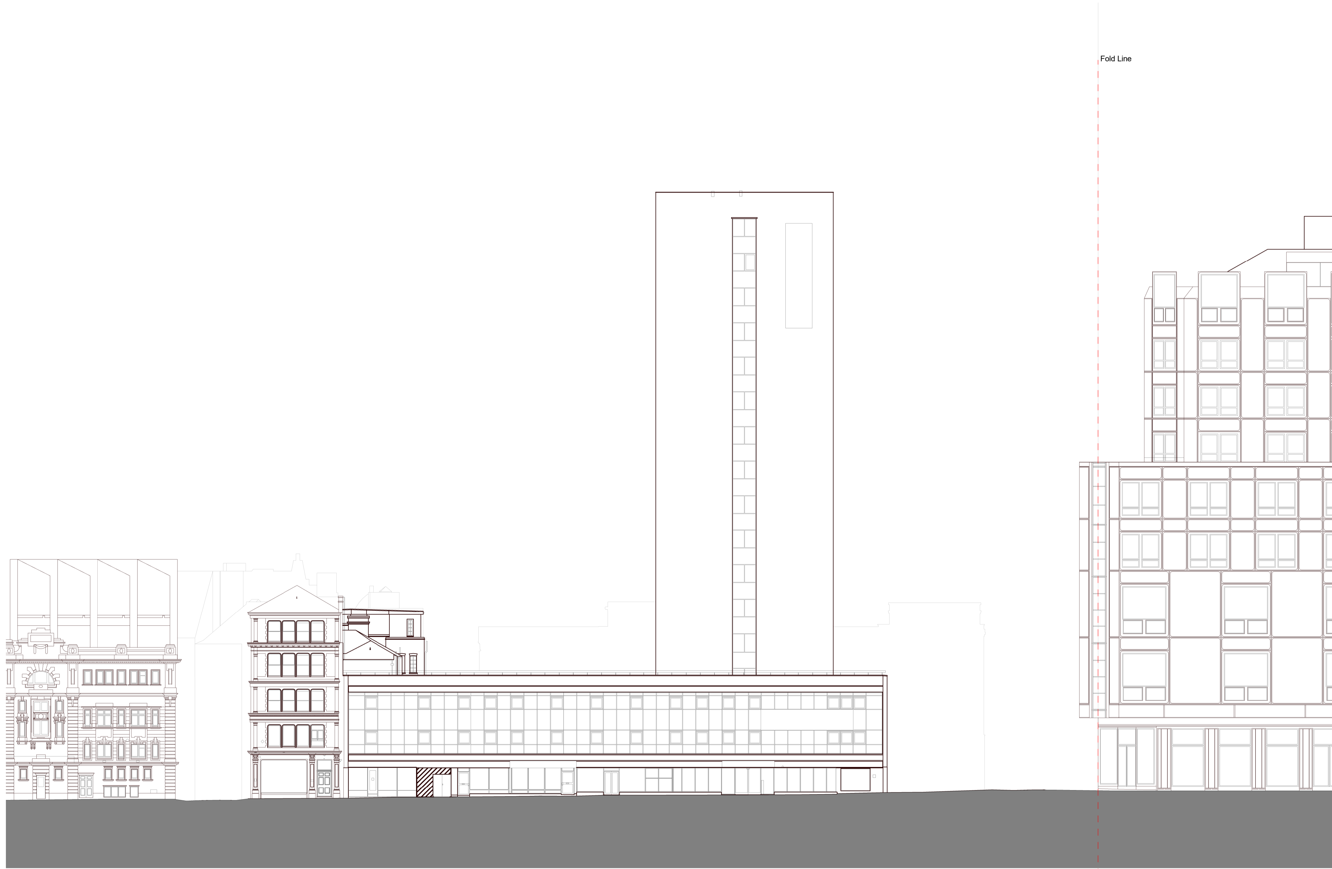
Shaftesbury Theatre Grape Street Cuban Embassy Site Extents Museum Street Post Building Existing High Holborn Elevation North
