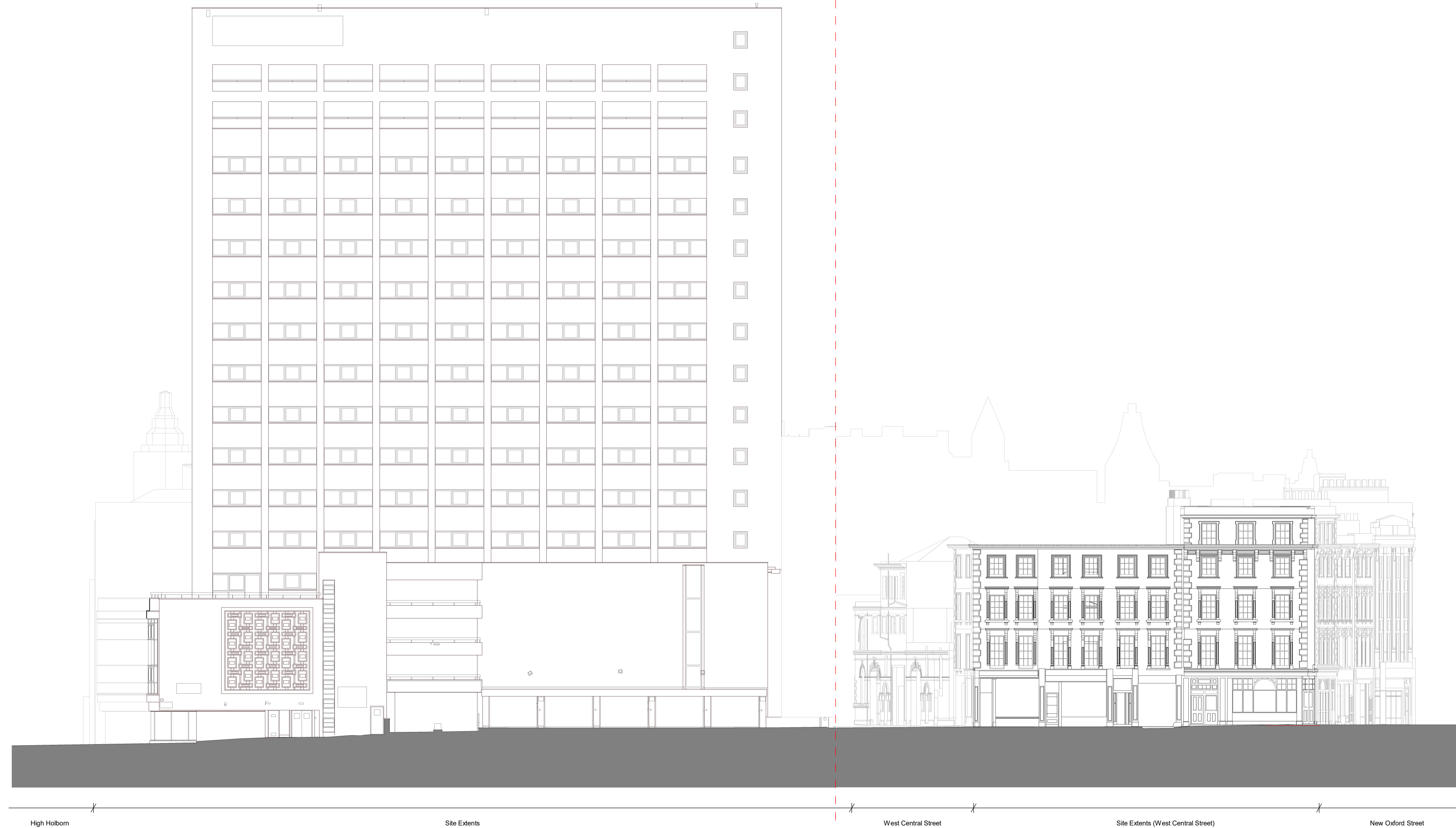
1 Existing Museum Street Elevation - West 1 : 200
