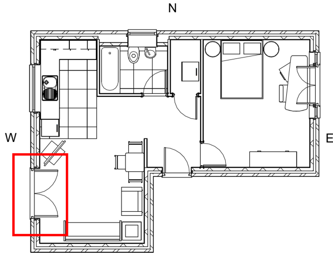
S PROPOSED FLOORPLAN
