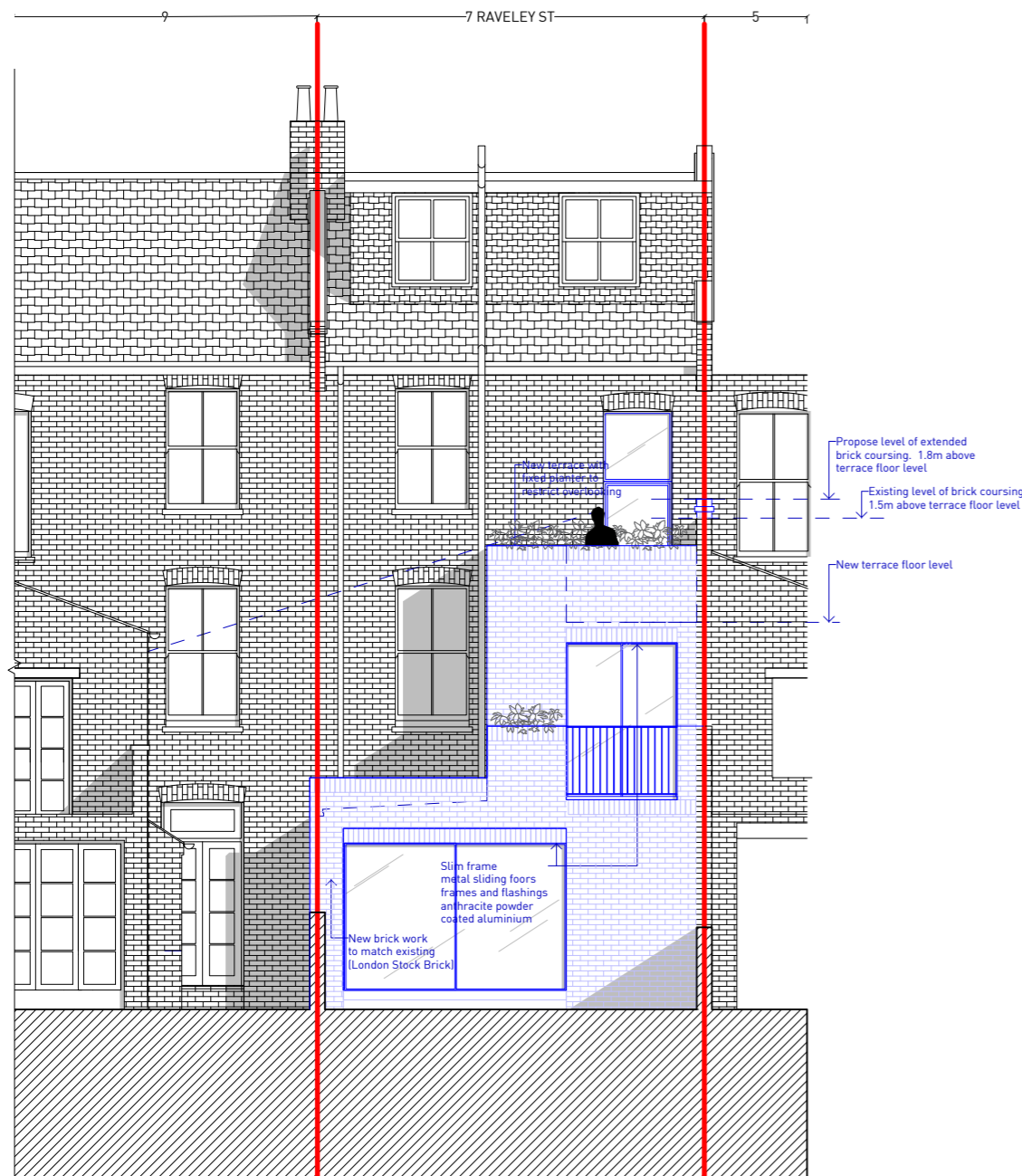
REAR ELEVATION
