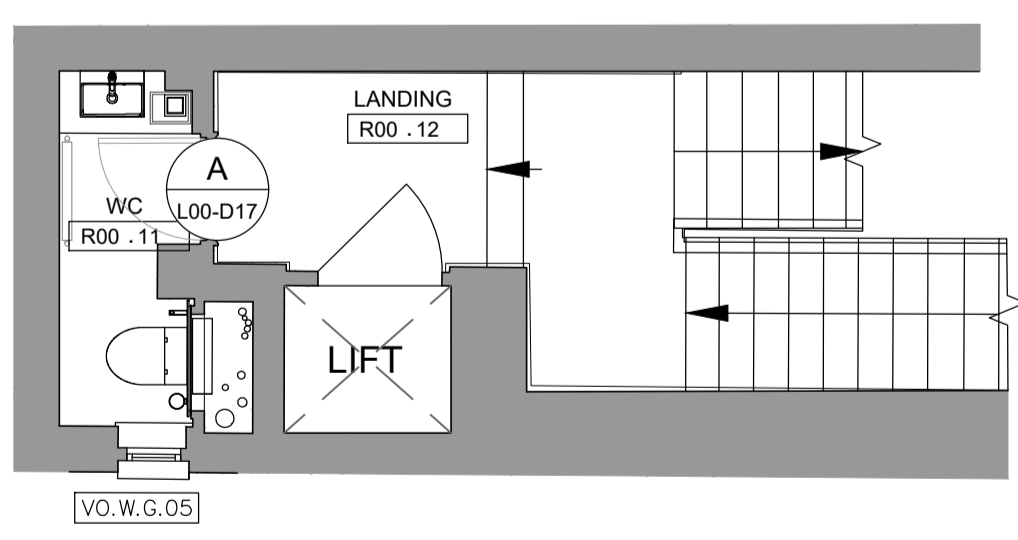
UPPER LANDING PLAN 1:50 @ A1
