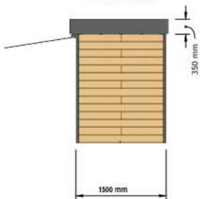
LEFT ELEVATION
