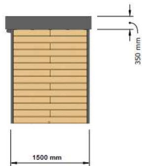
LEFT ELEVATION
