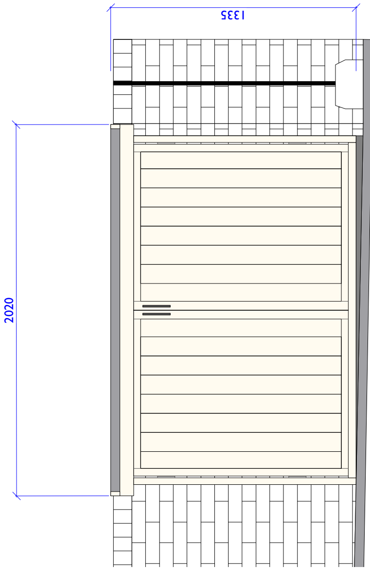
FRONT ELEVATION scale 1:20
