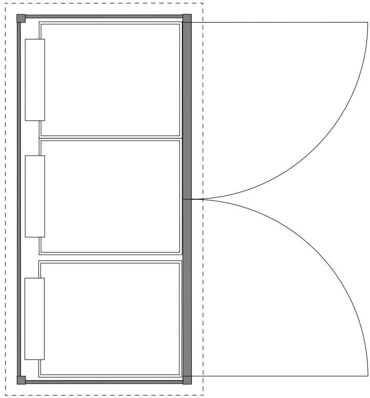
PLAN, scale 1:20
