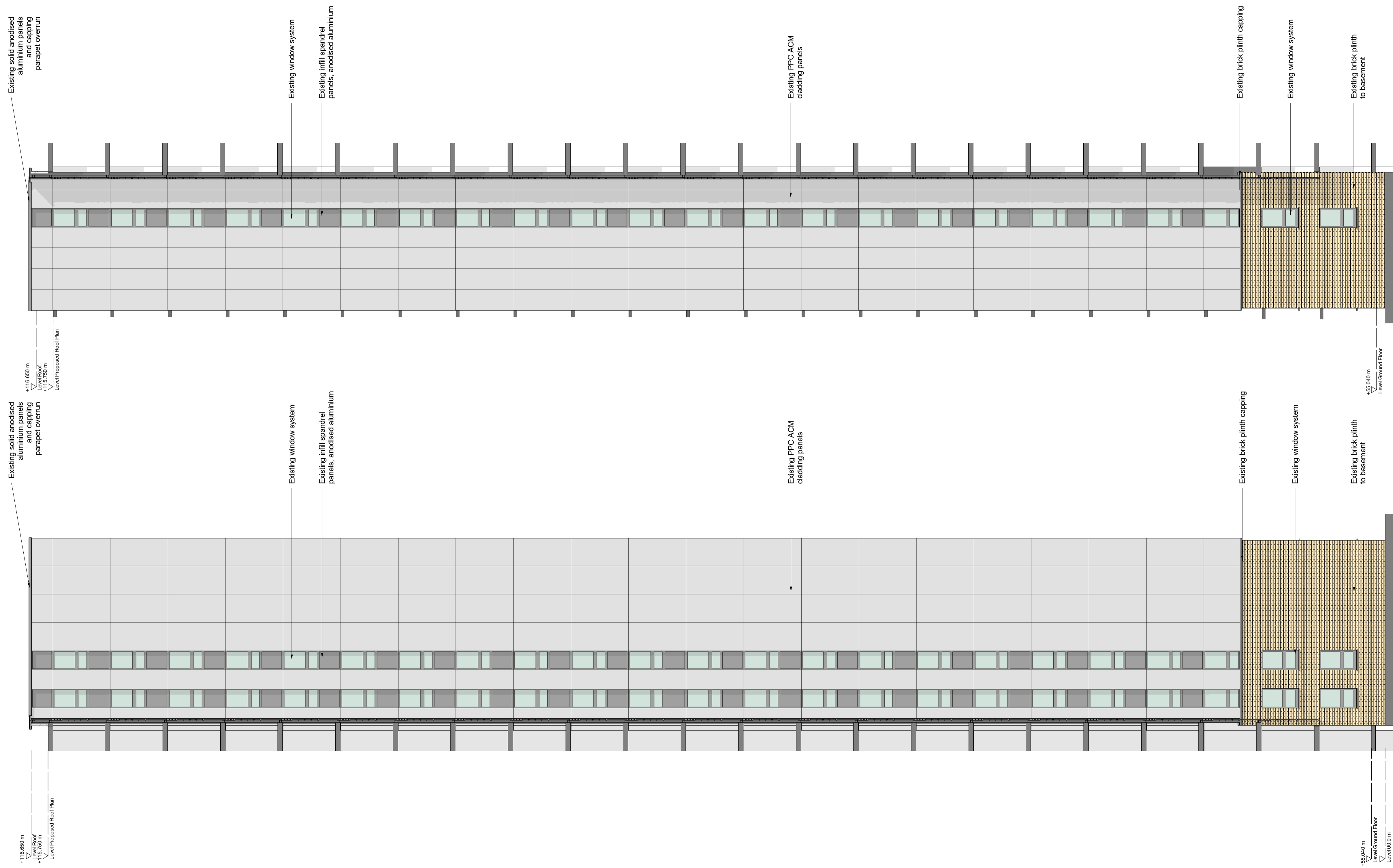
2-Elevation - Internal East Scale 1 : 100
