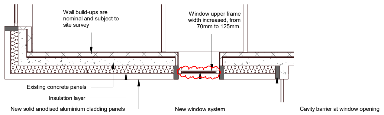
3 2F - Detailed Plan 4 1 : 50
