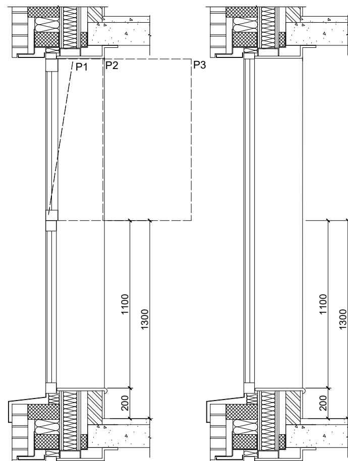
SECTION C-C
