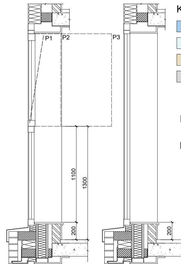
SECTION E-E
