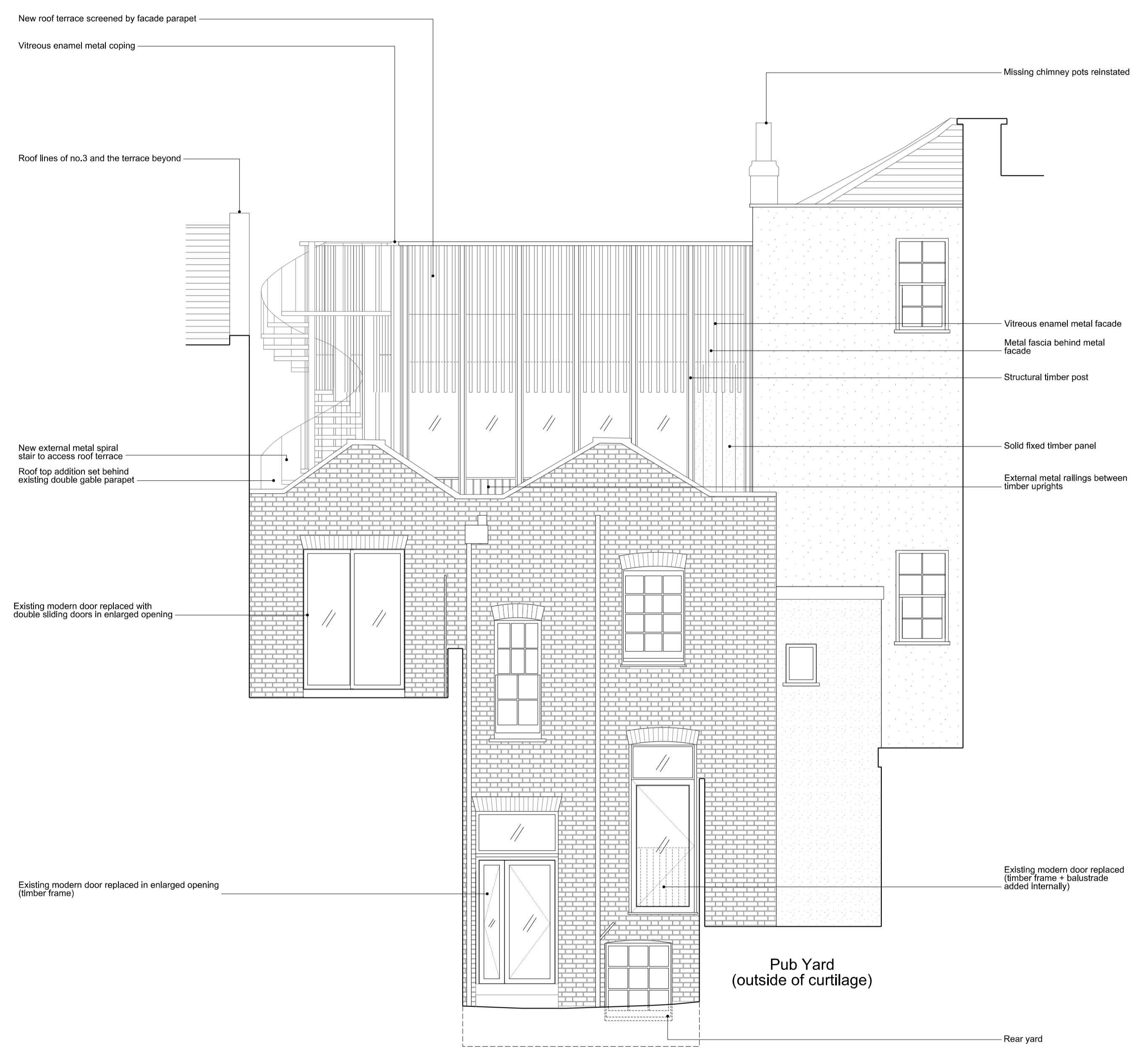
Rear Elevation
