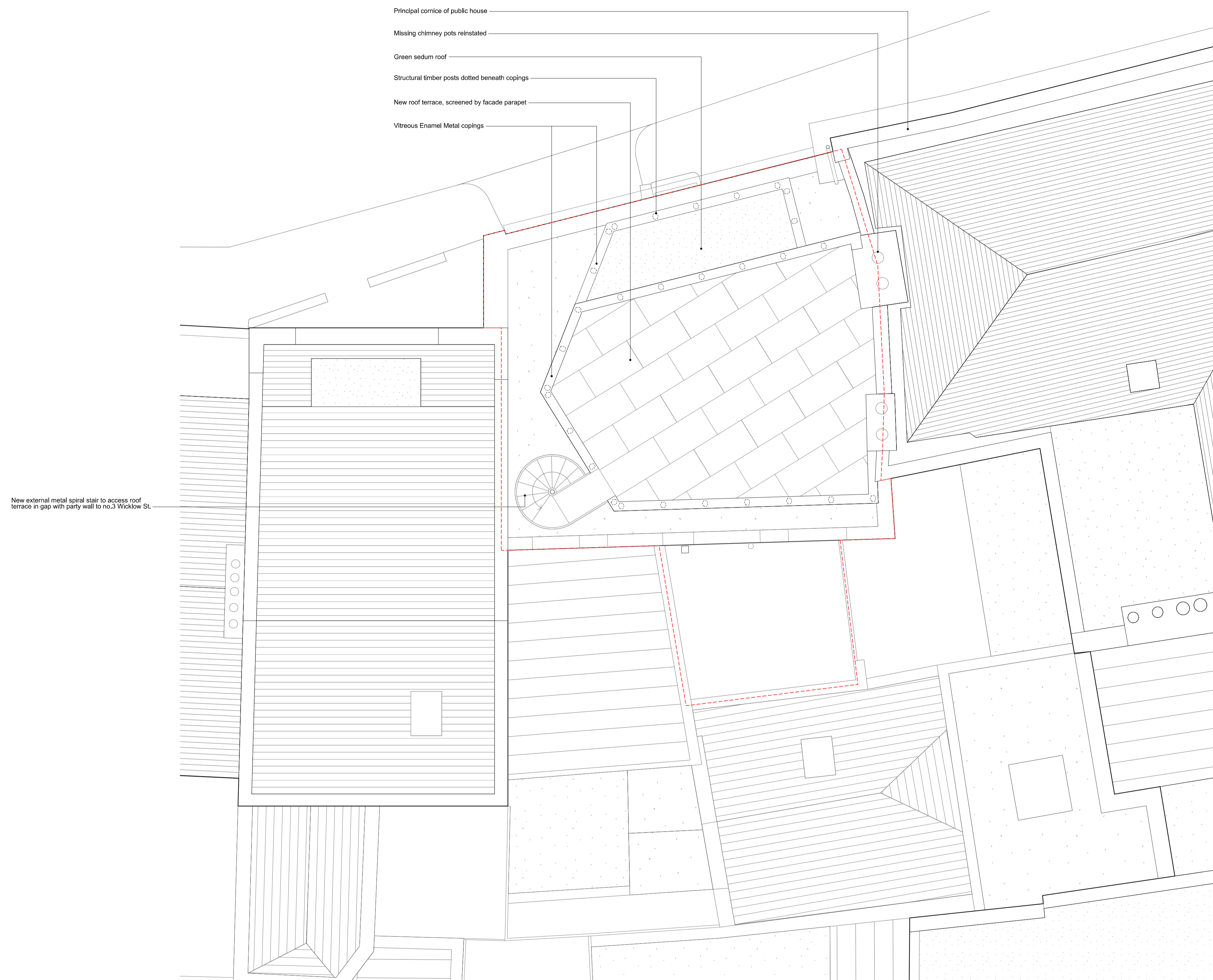
Roof Plan
