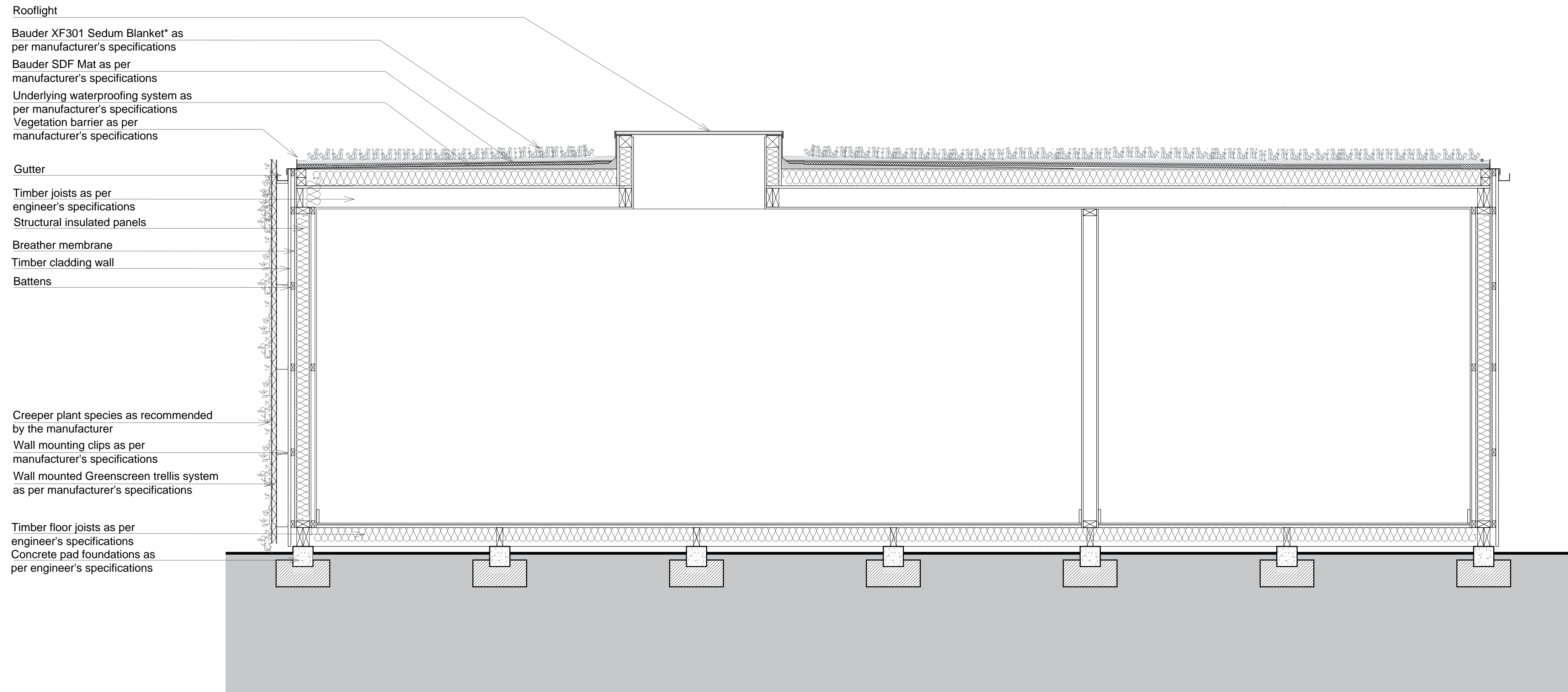
Detail Section Scale 1:20
