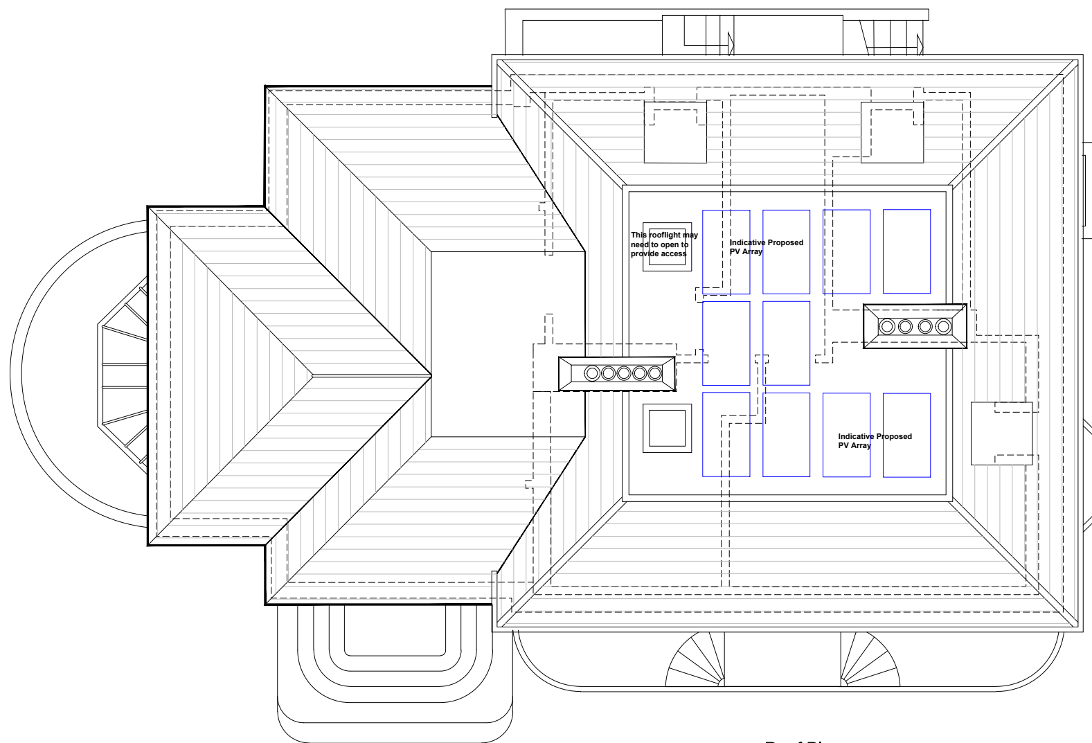
Roof Plan
