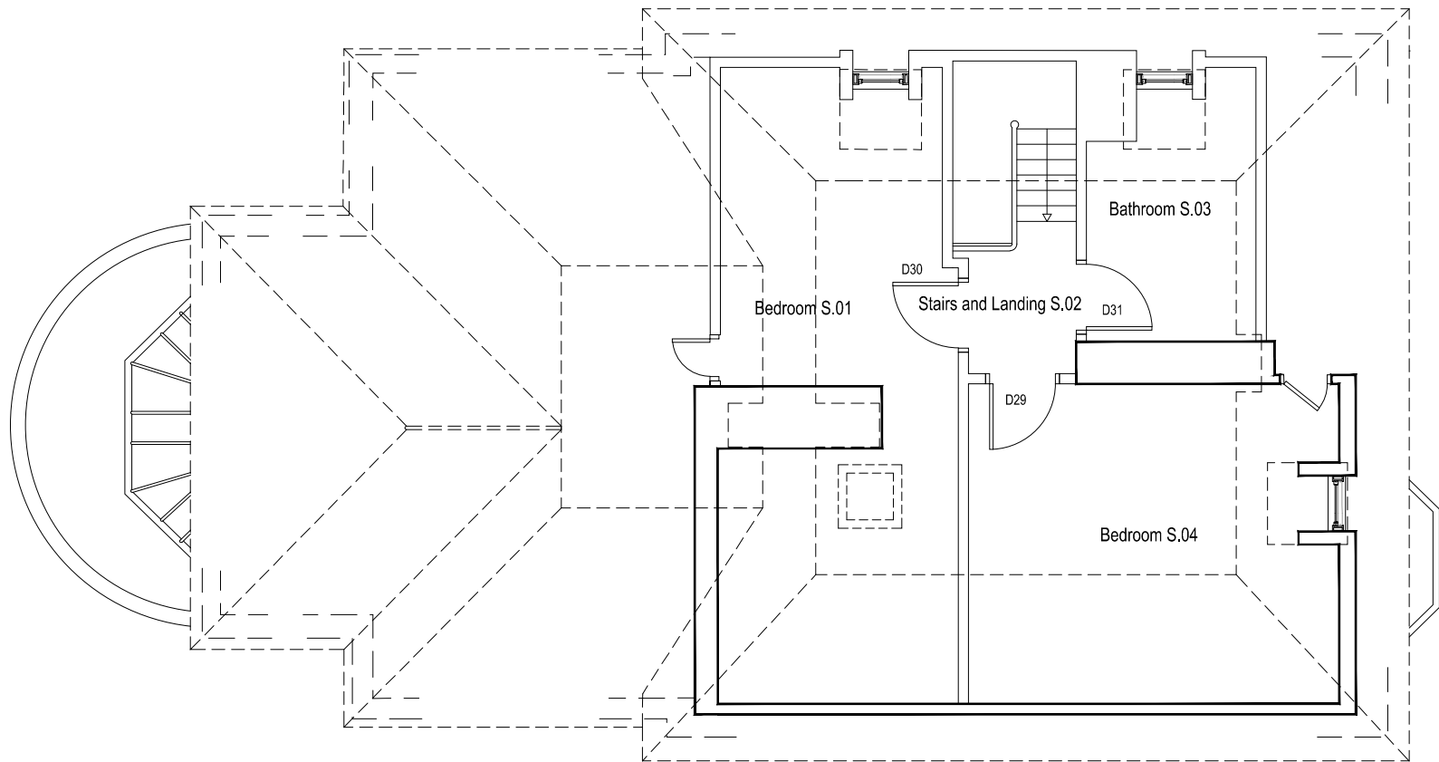
2 nd Floor Plan has no changes proposed
