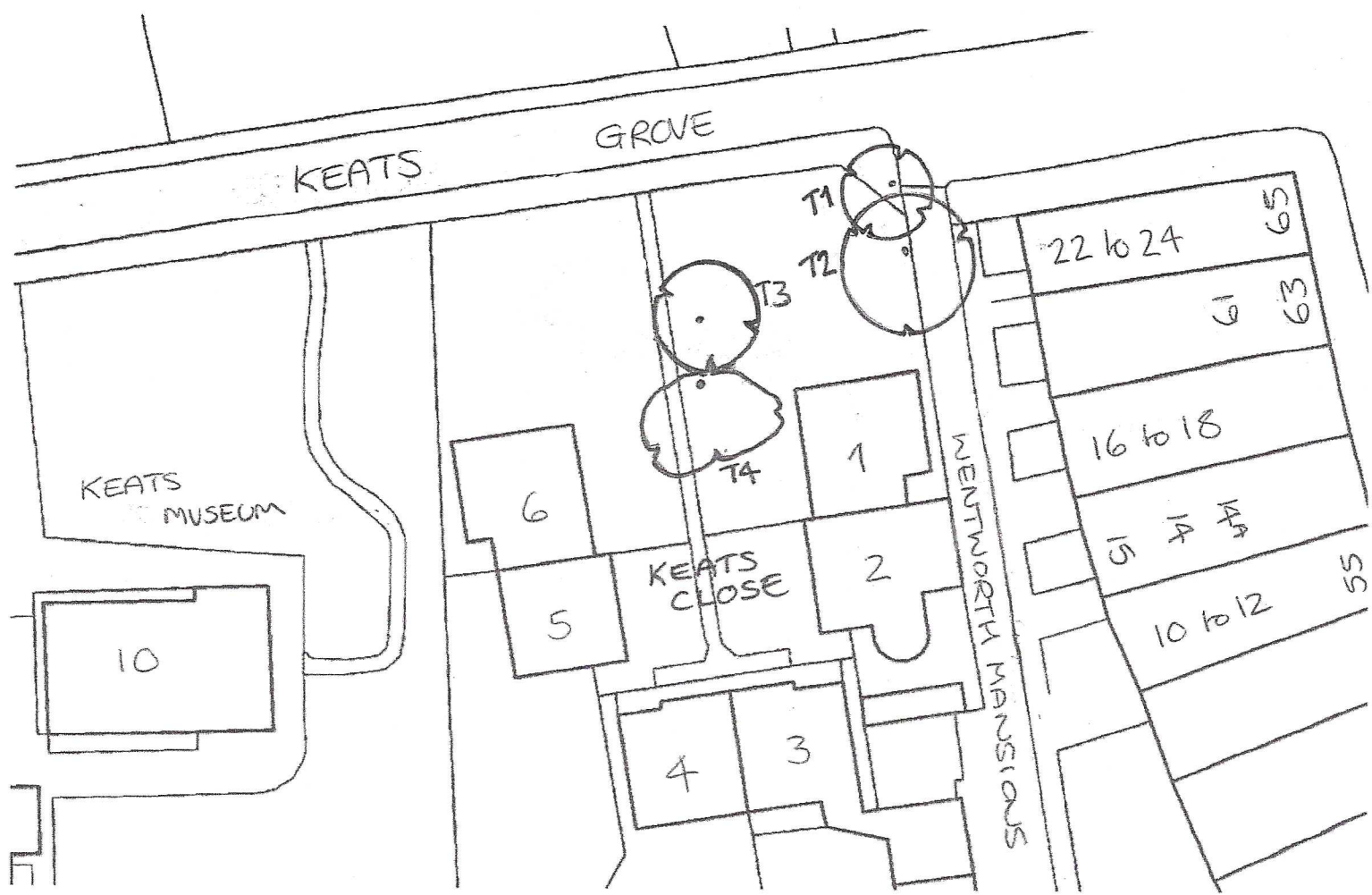
SITE PLAN FOR 1, KEATS CLOSE, LONDON, NW3 2RP
