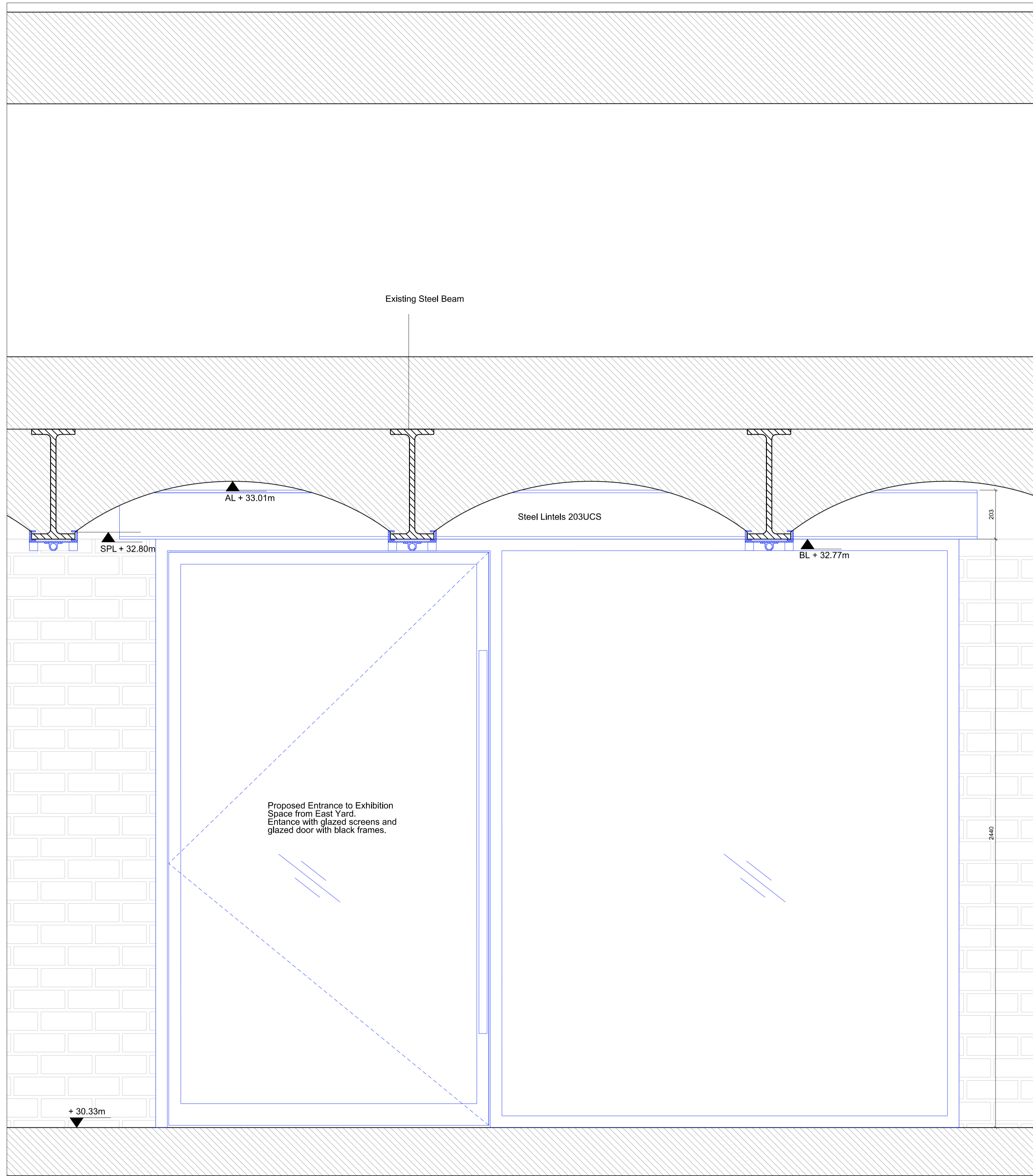
01 ENTRANCE FROM WEST YARD PROPOSED ELEVATION
