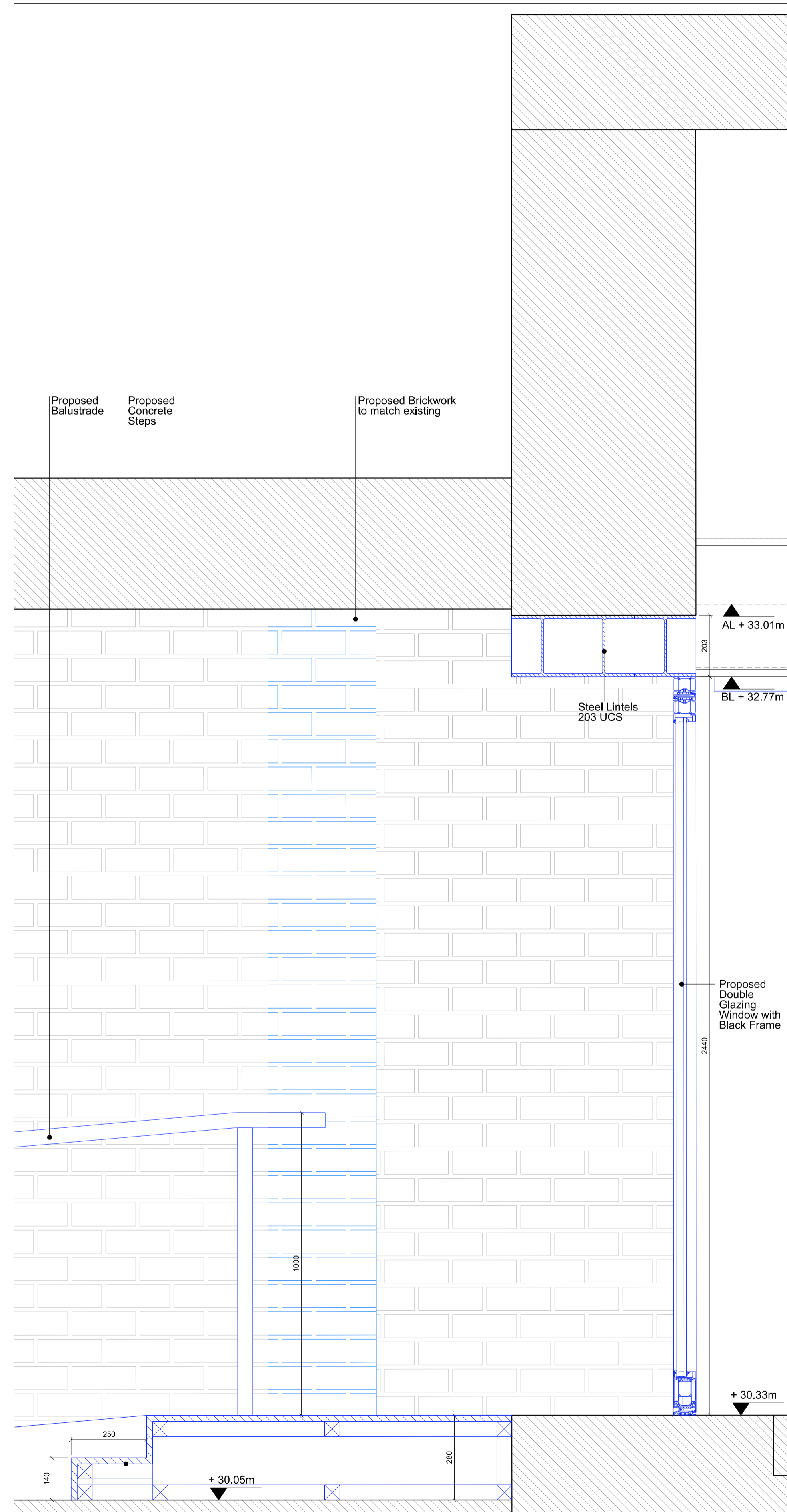
02 ENTRANCE FROM WEST YARD PROPOSED SECTION
