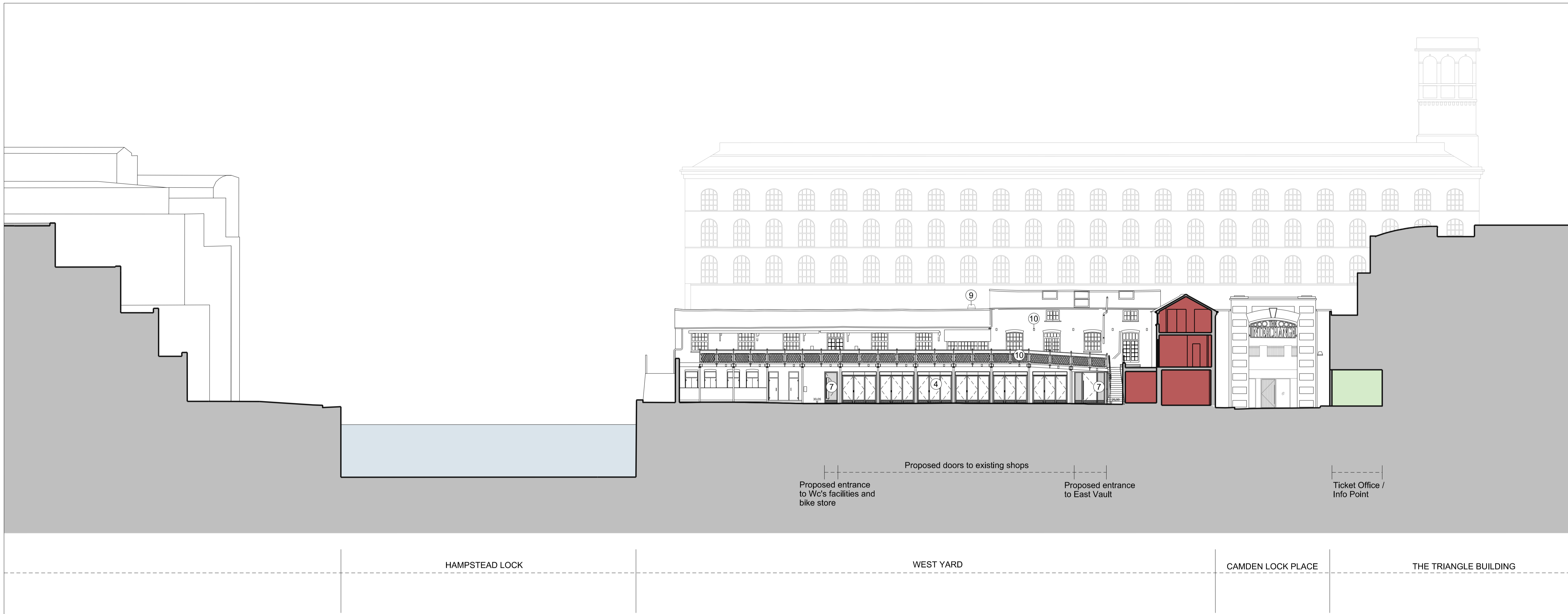
01 SECTION C-C 1:200 at A1
