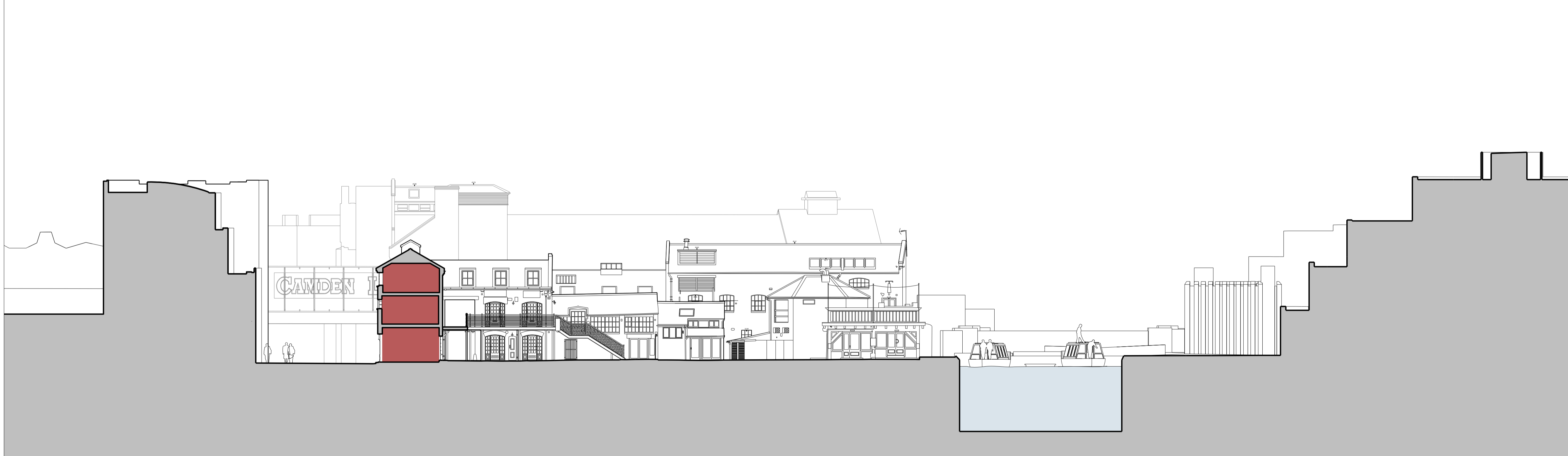
02 SECTION D-D 1:200 at A1
