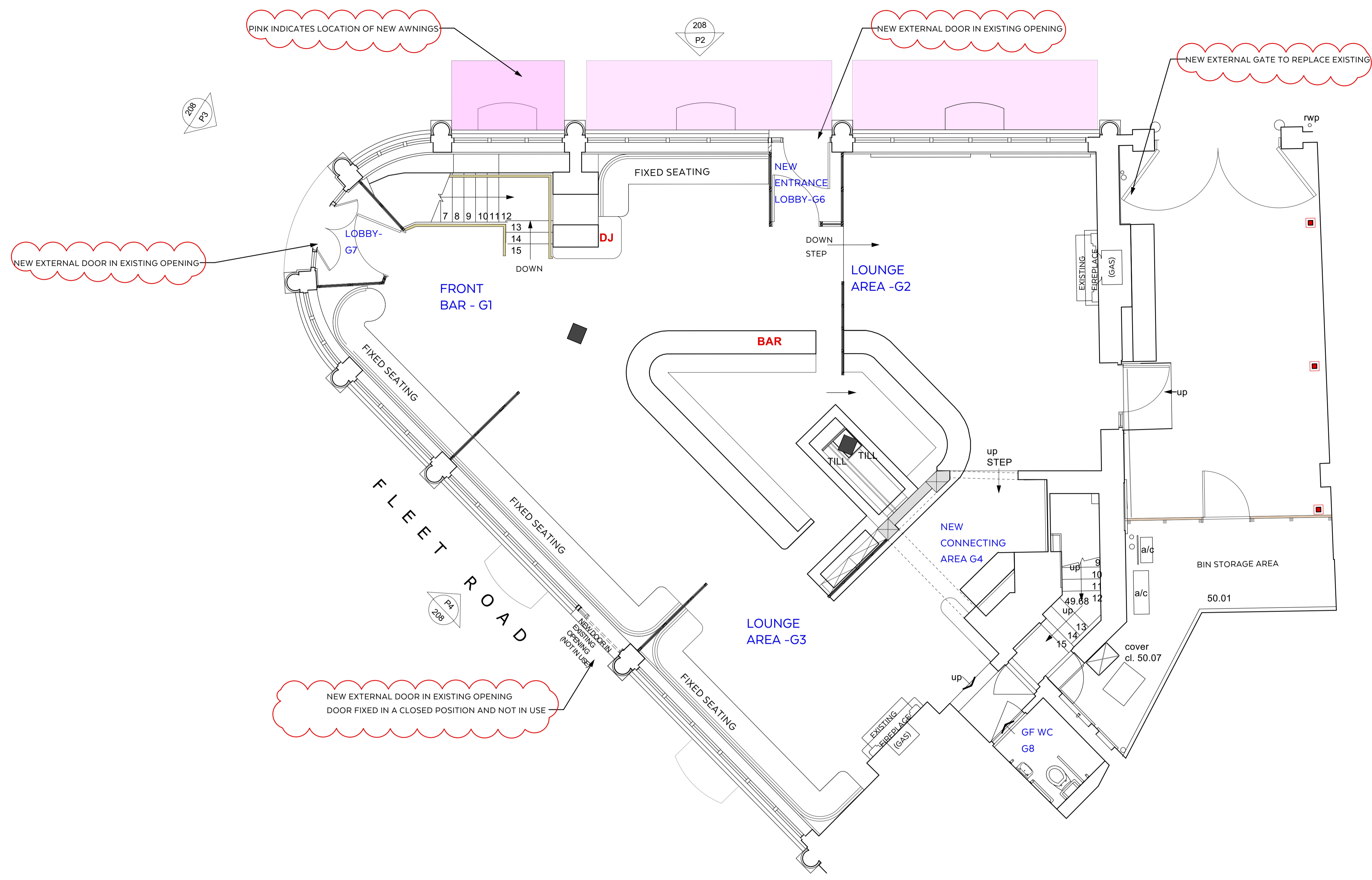
GPP GROUND FLOOR PROPOSED PLAN Scale: 1:50
