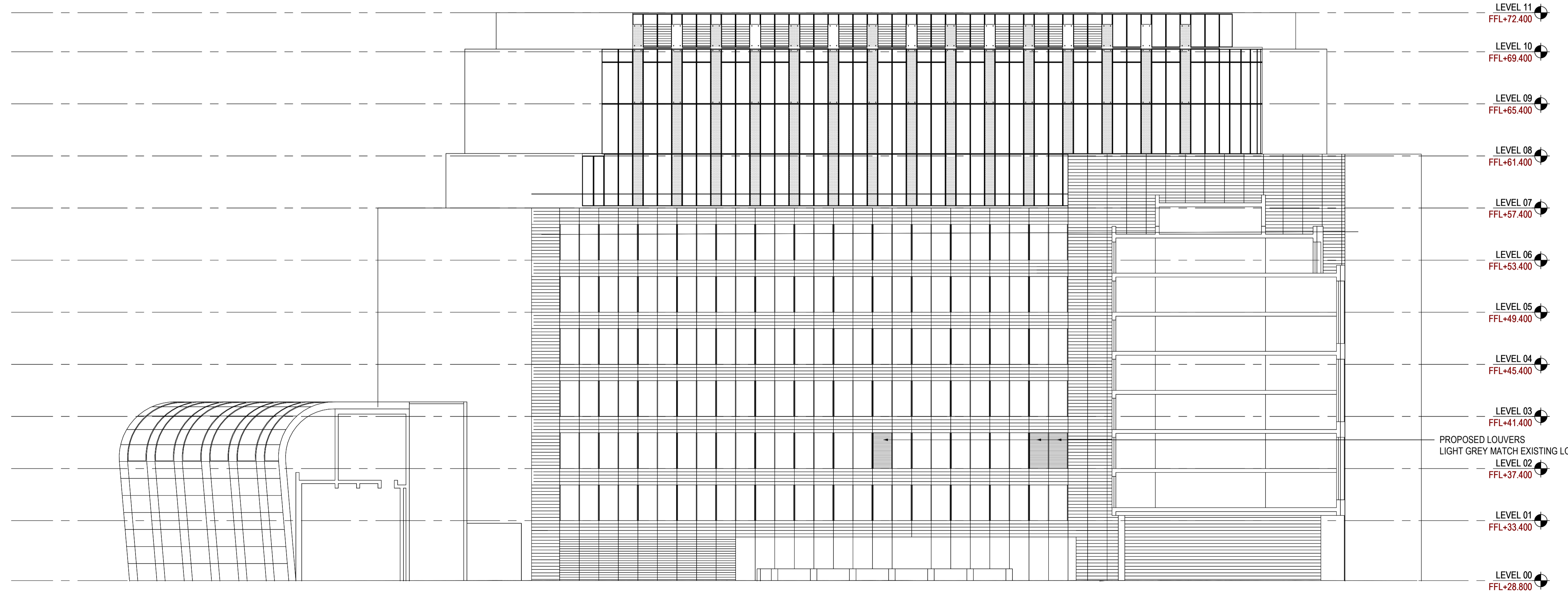
01 ELEVATION NORTH_PROPOSED SCALE: 1:200
