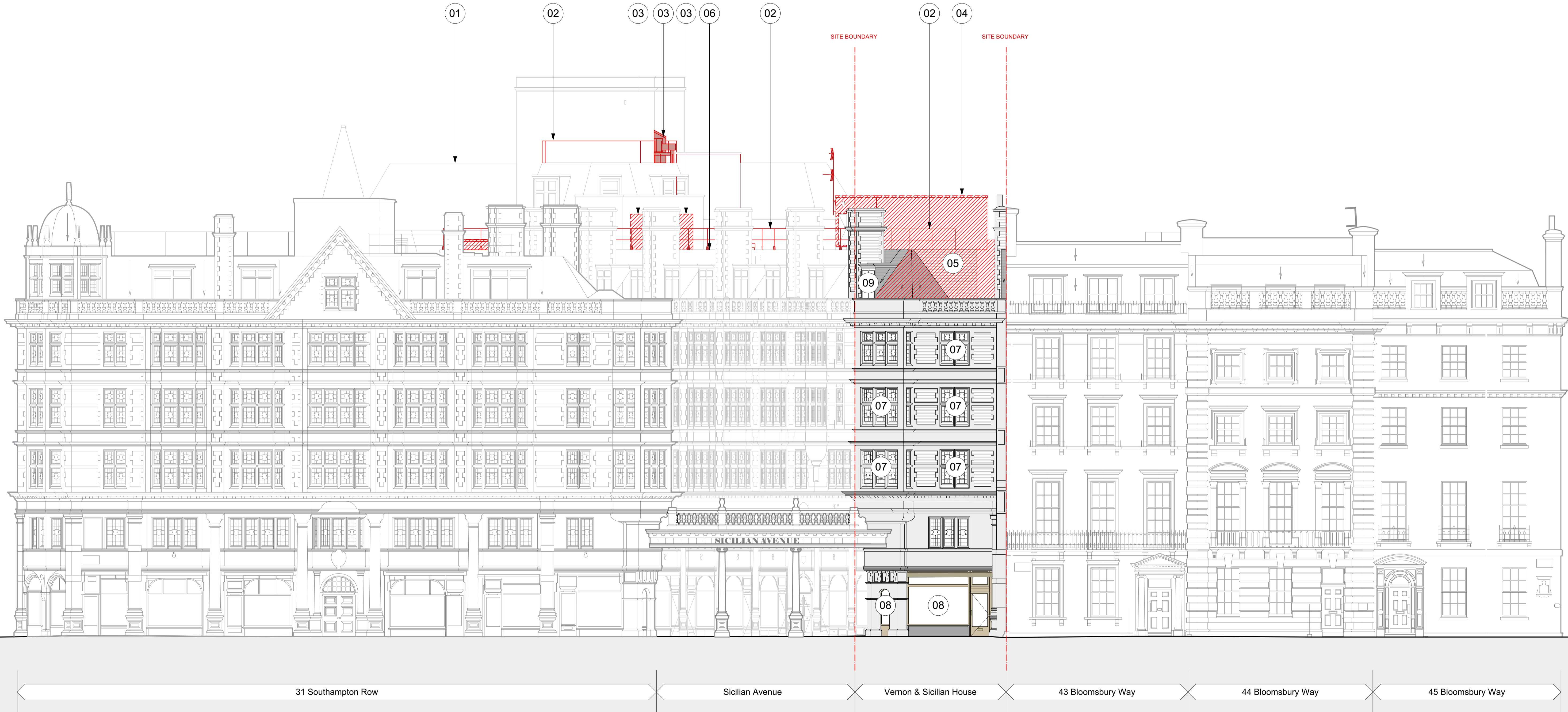
1 Vernon & Sicilian House Demolition North West Context Elevation Scale: 1:100
