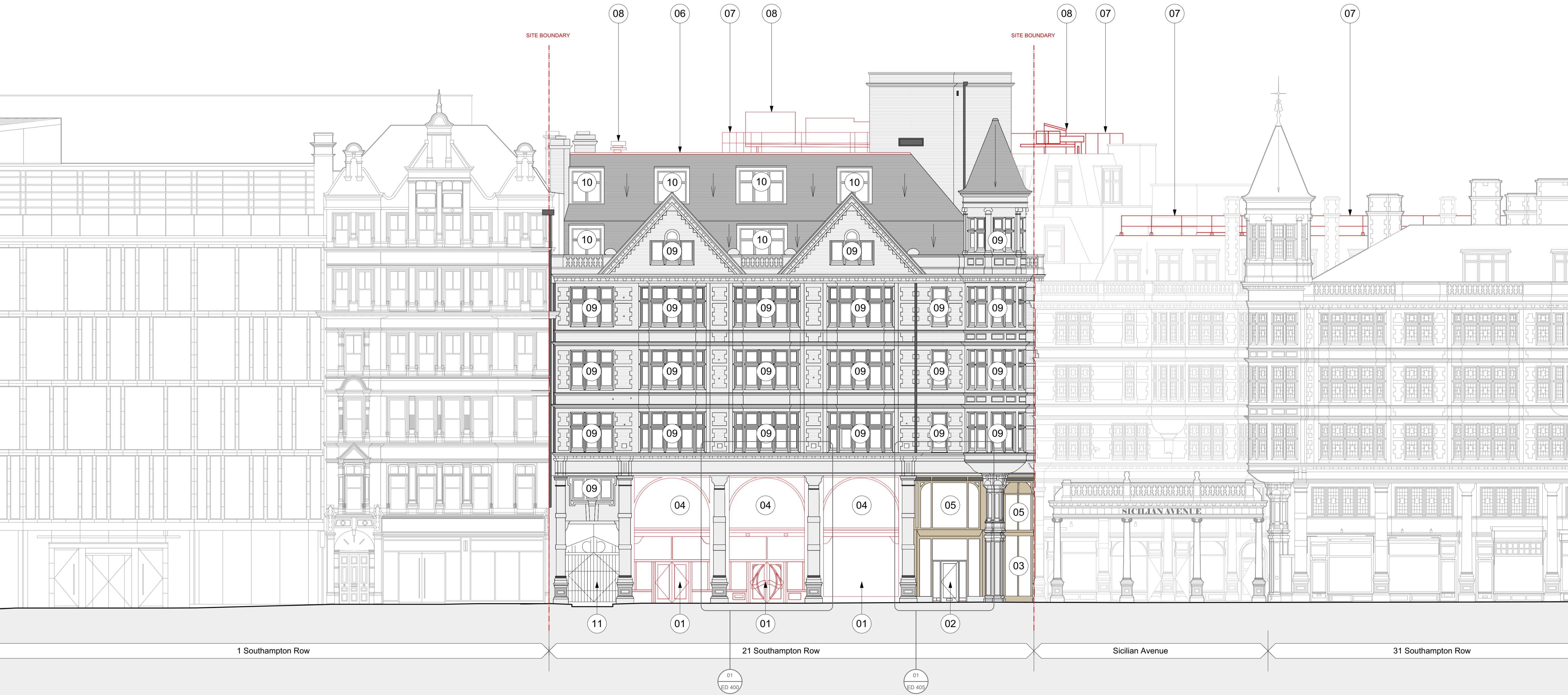
1 21SR Demolition East Context Elevation Scale: 1:100
