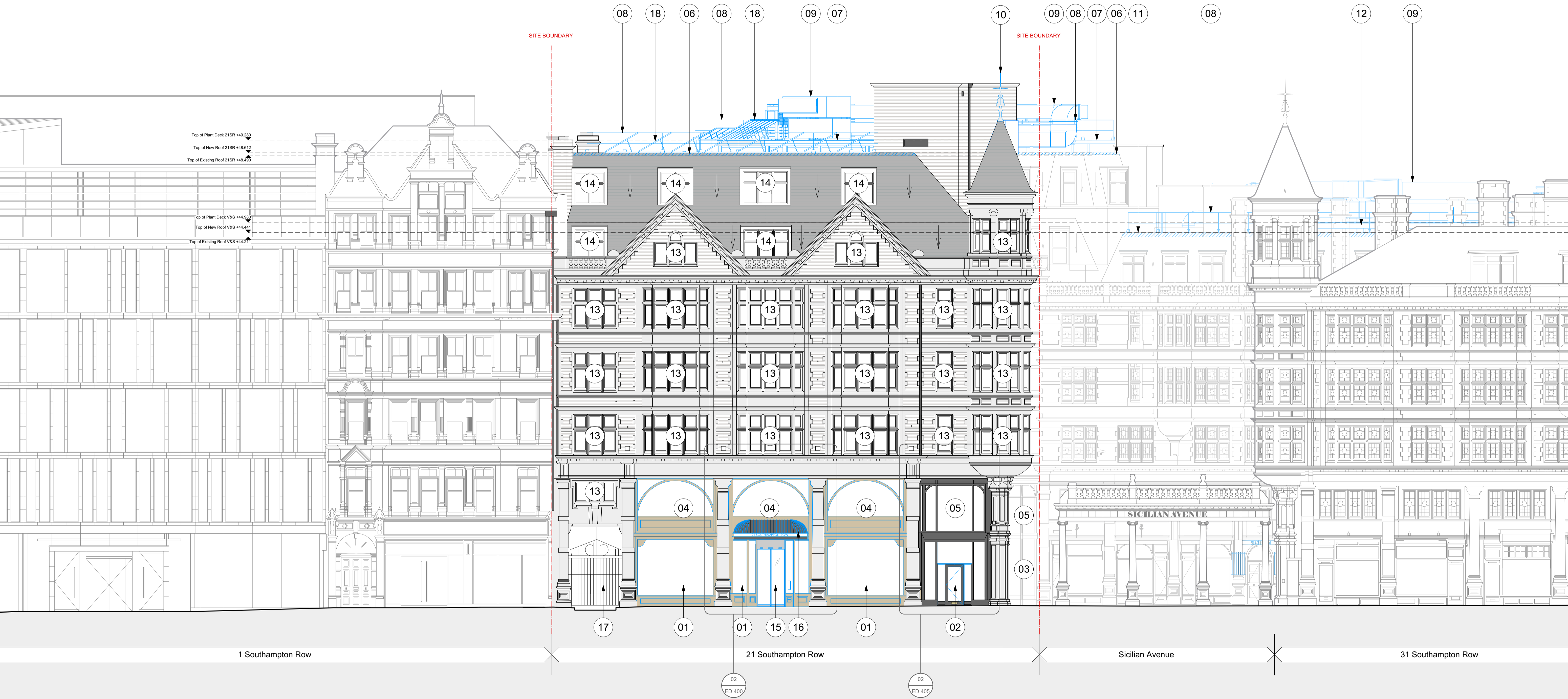
1 21SR Proposed East Context Elevation Scale: 1:100
