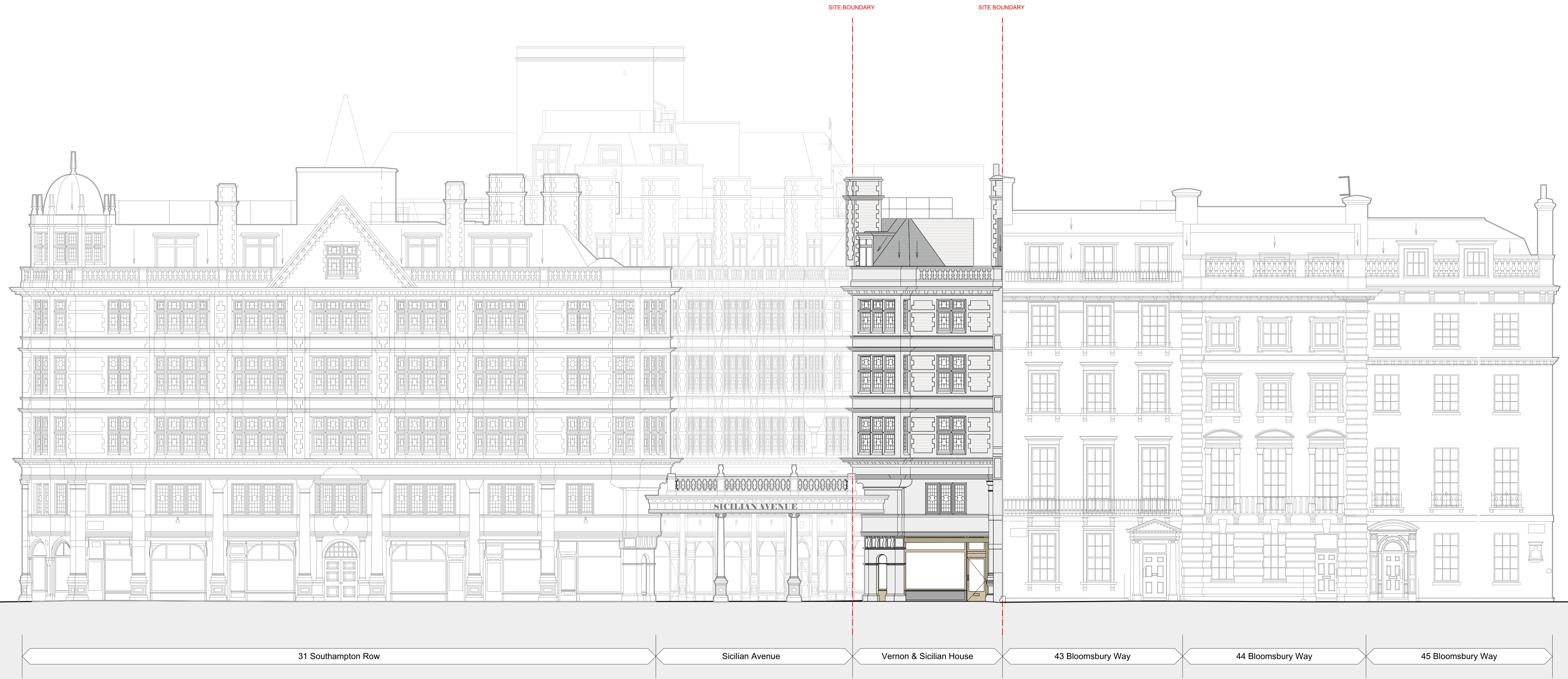
1 Vernon & Sicilian House Existing North West Context Elevation Scale: 1:100
