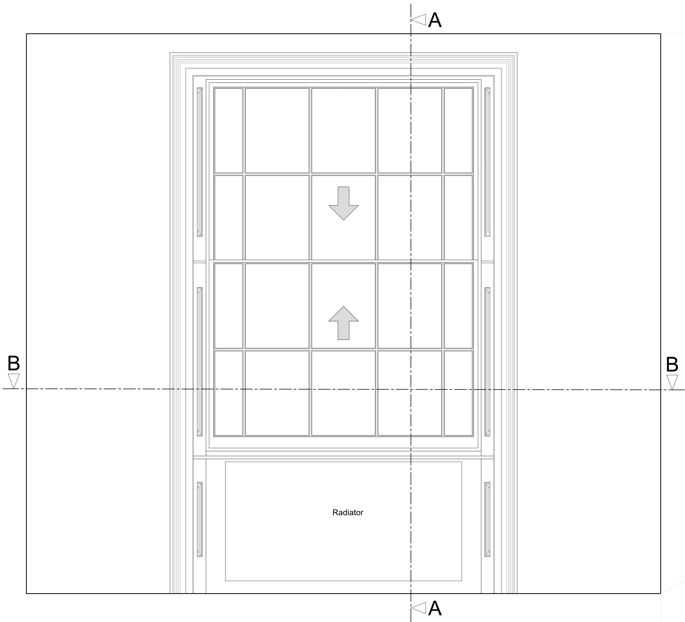
Internal Room Elevation Scale: 1:10
