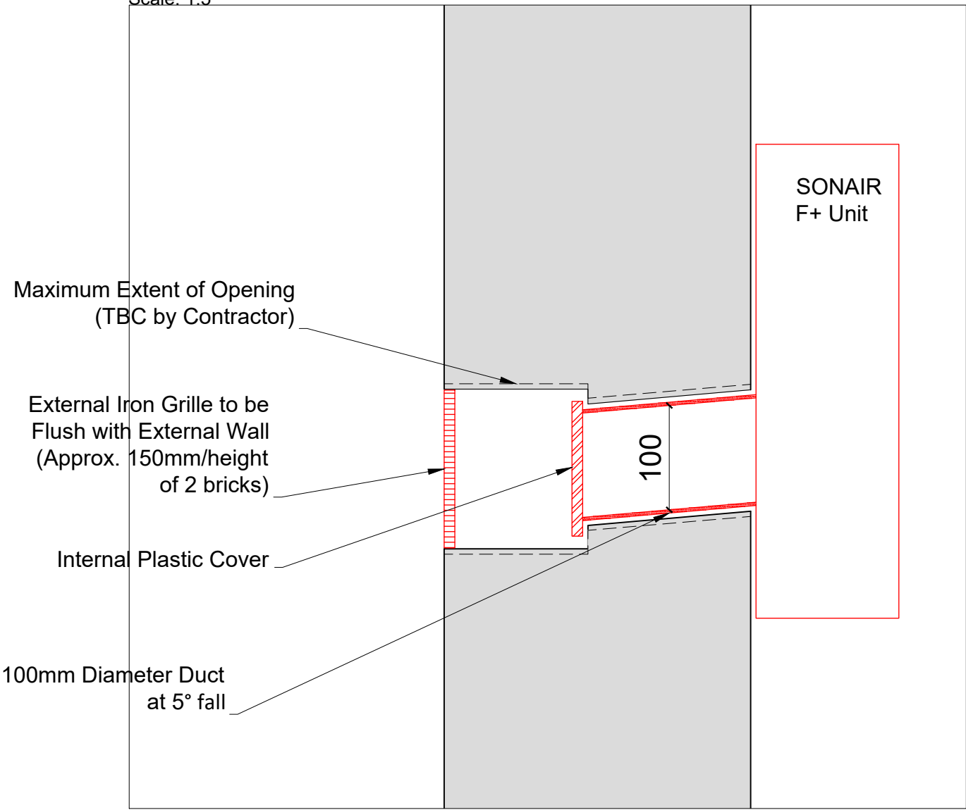
Detail of Sonair Unit Scale: 1:5
