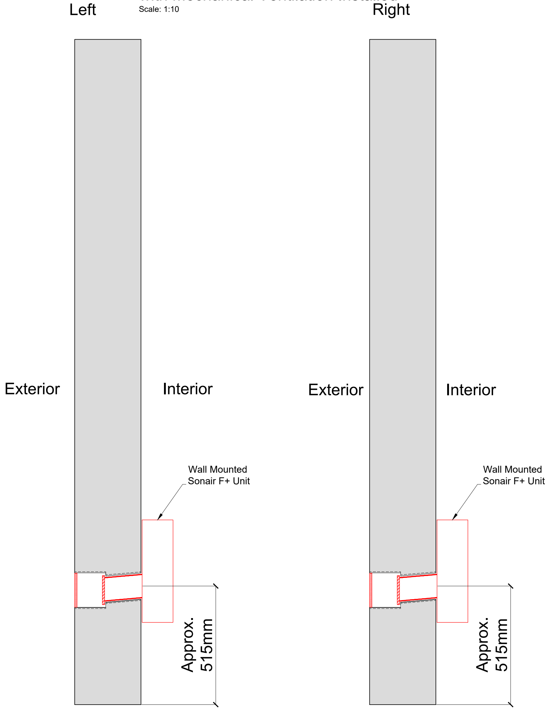
Section H-H through External Wall with Mechanical Ventilation Installed Scale: 1:10
