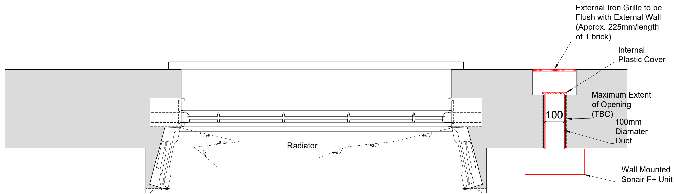
Plan Section B-B with Secondary Glazing Installed
