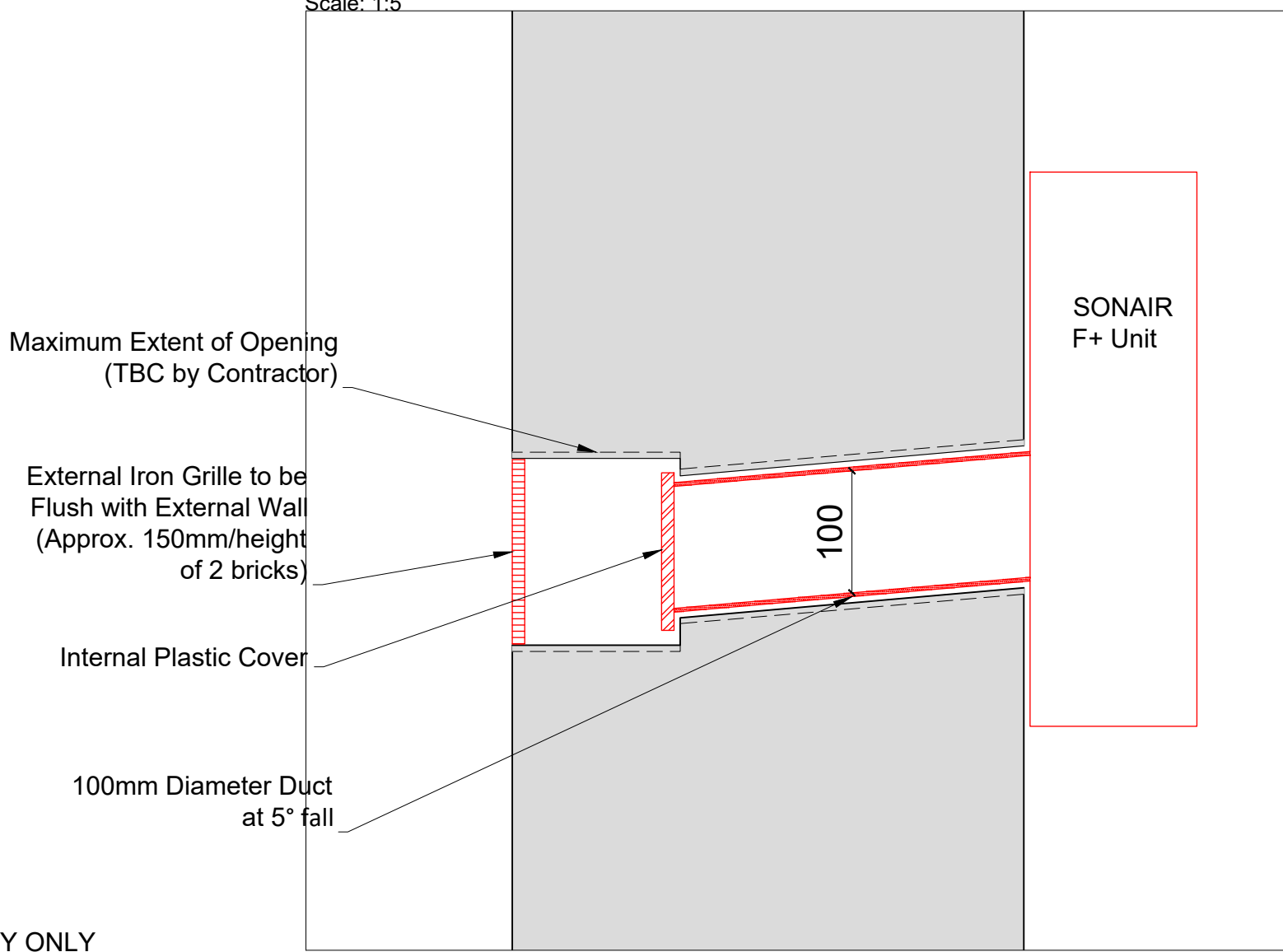
Detail of Sonair Unit
