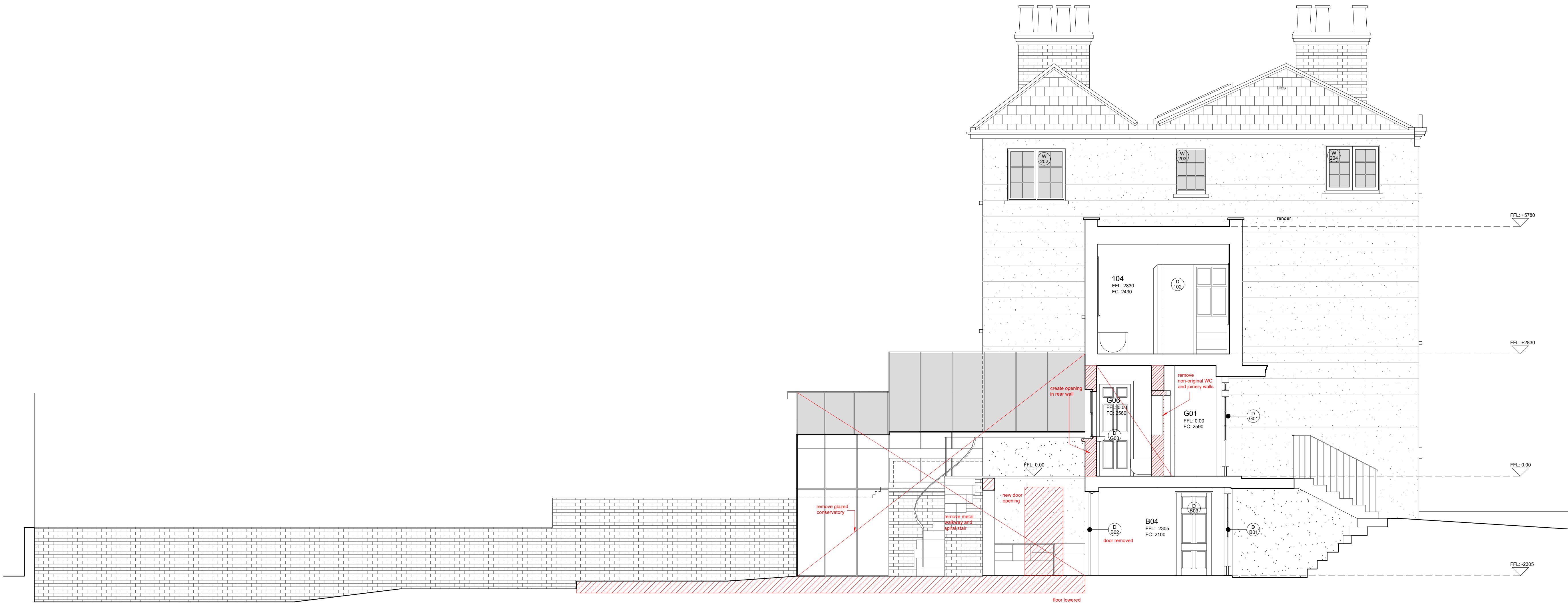
Section 1-1
