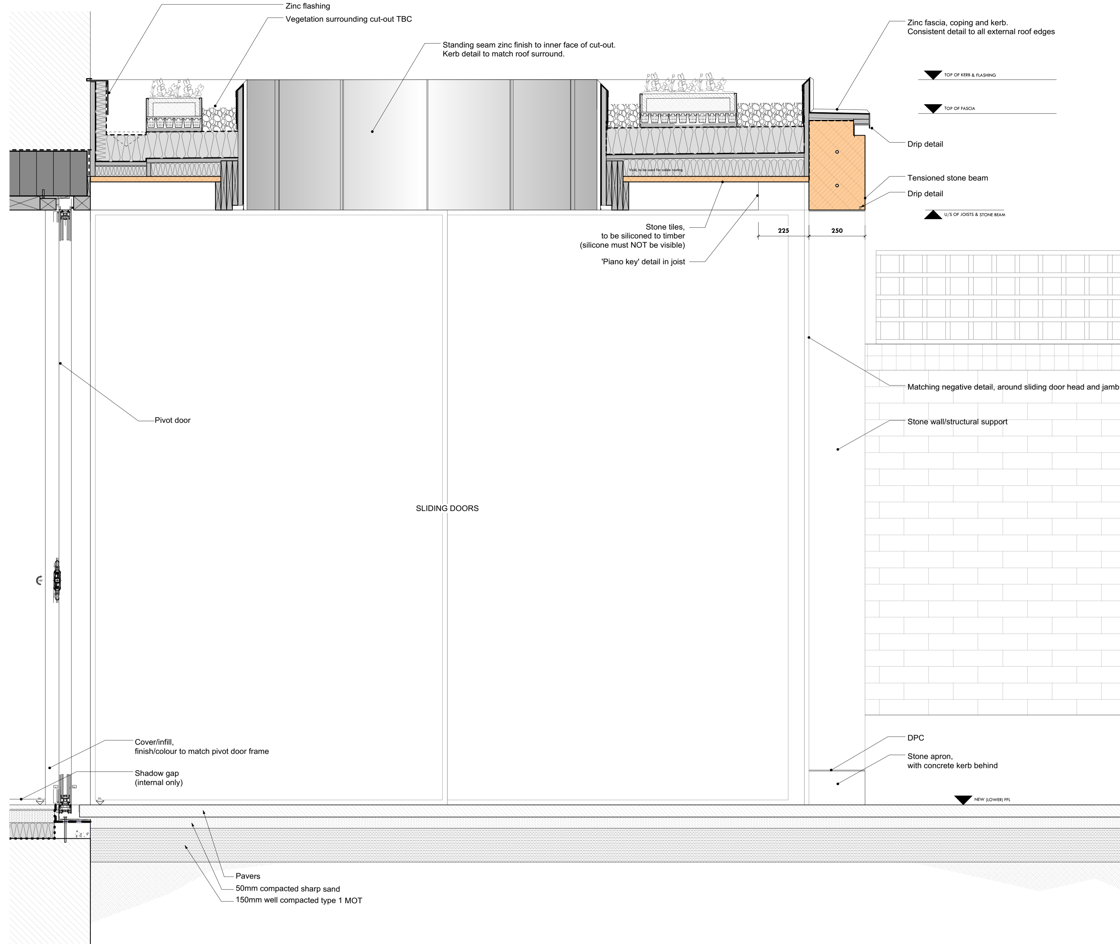
1 EXTENSION 186 SECTION 1:10
