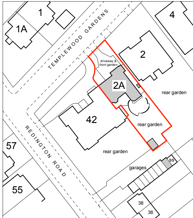
LOCATION PLAN 1:1250
