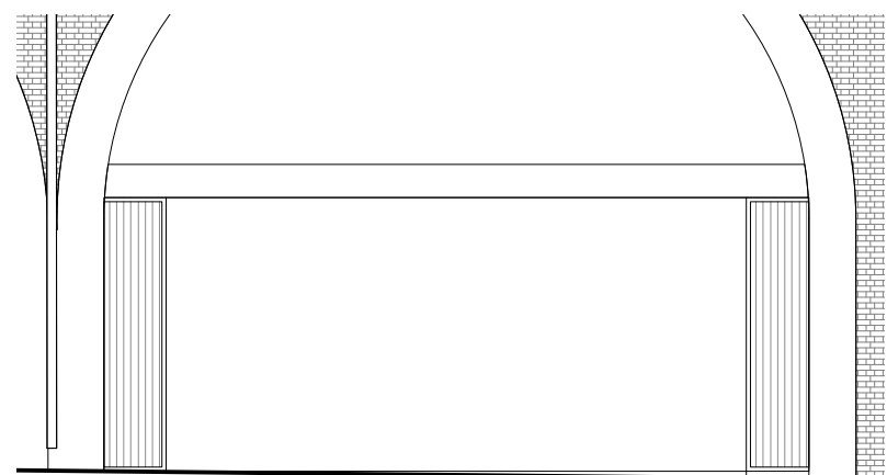
3 Elevation: Gate in Open Configuration 1:100
