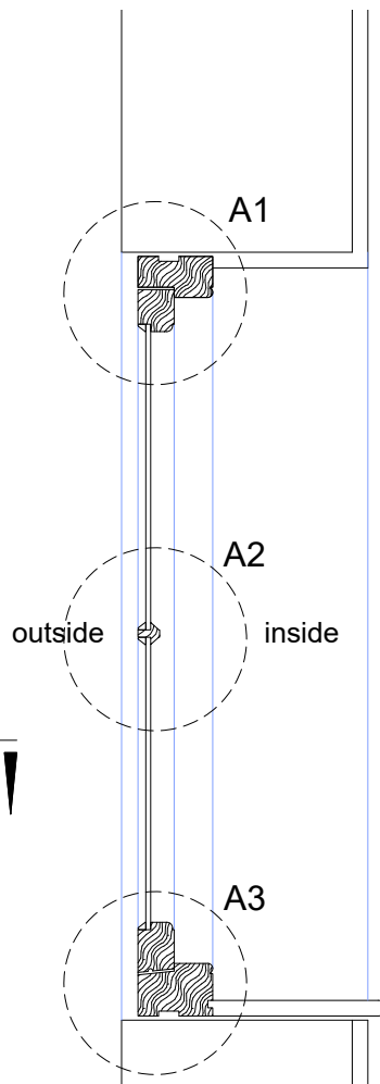
Section AA
