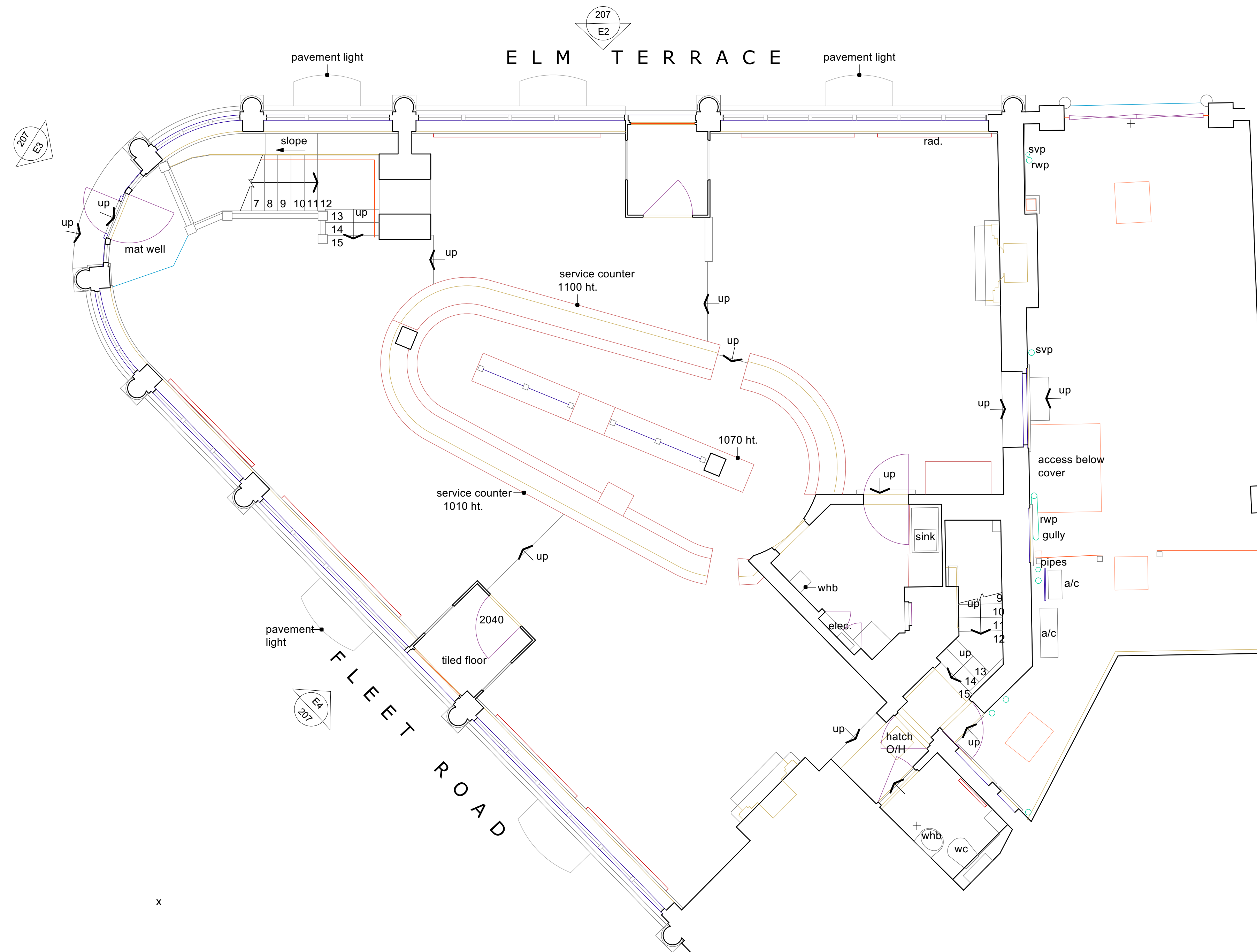
GEP GROUND FLOOR EXISTING PLAN Scale: 1:50
