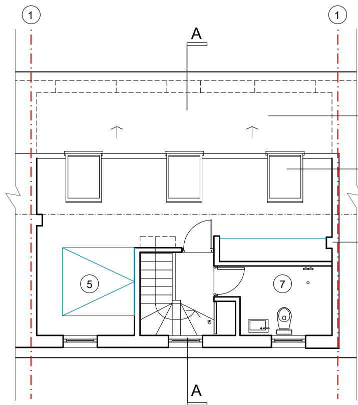
SECOND FLOOR PLAN - SCALE 1:100
