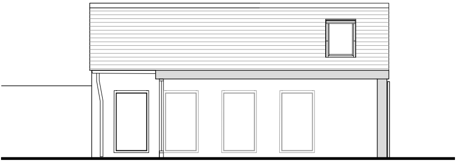
Eastern Sectional Elevation
