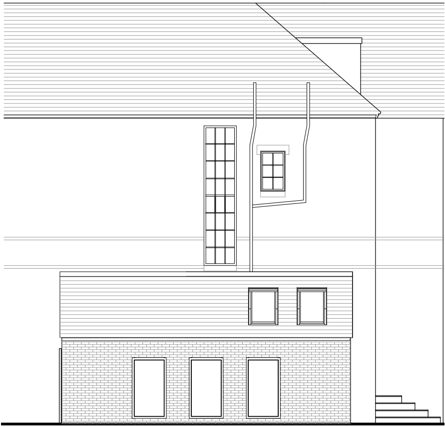
Western Elevation
