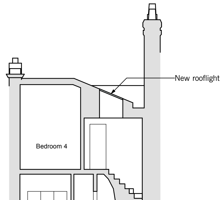
3. PROPOSED SECTION CC
