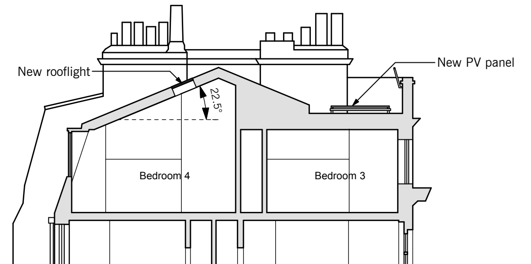
2. PROPOSED SECTION BB
