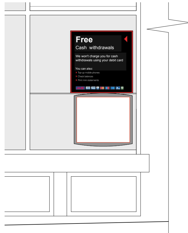
01 Ext Machine Detail Plan 1:25@A3
