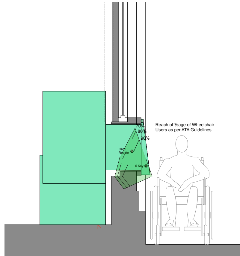
03 Ext Machine Detail Section 1:25@A3
