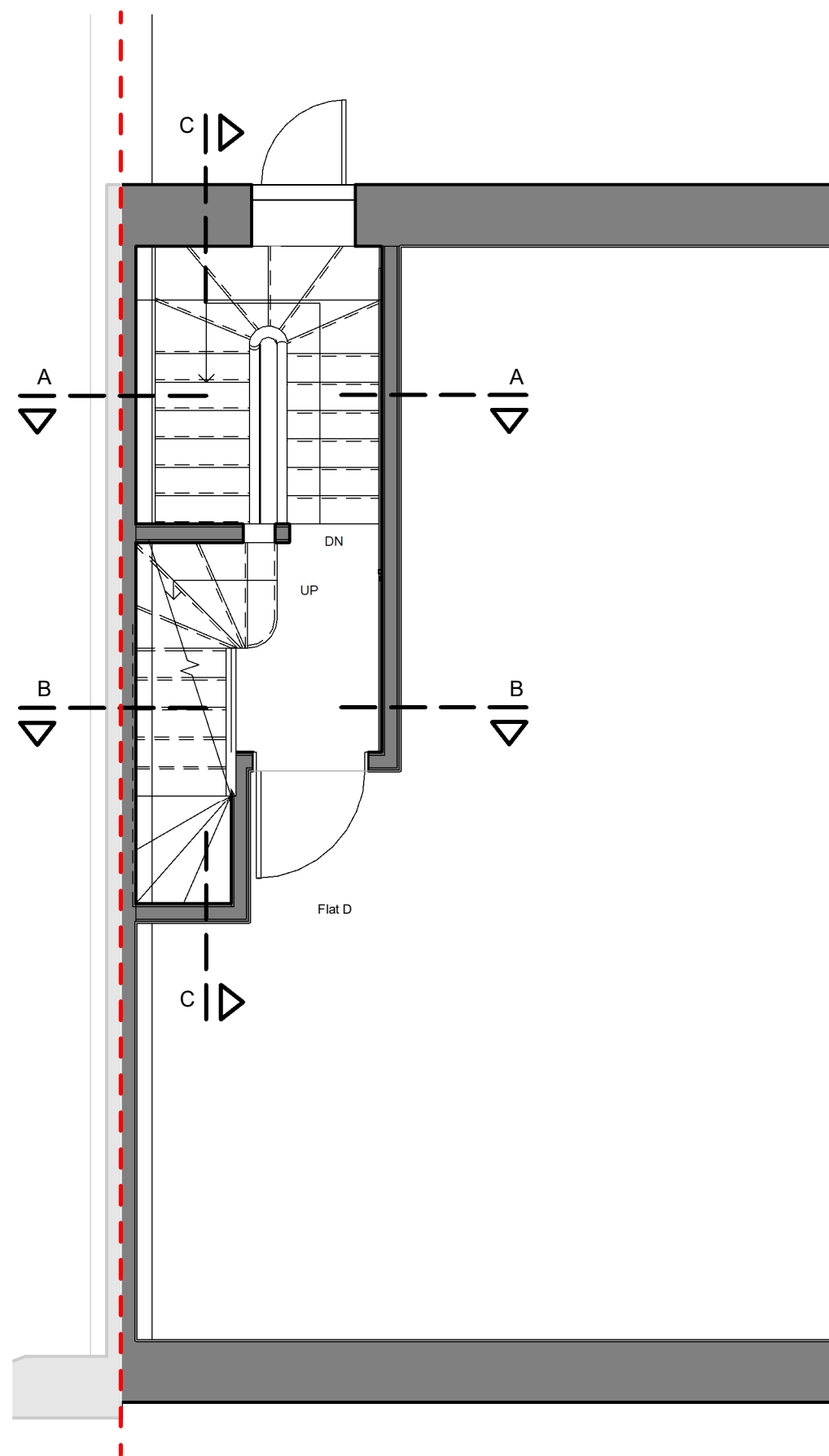
① Existing Second Floor 1 : 50
