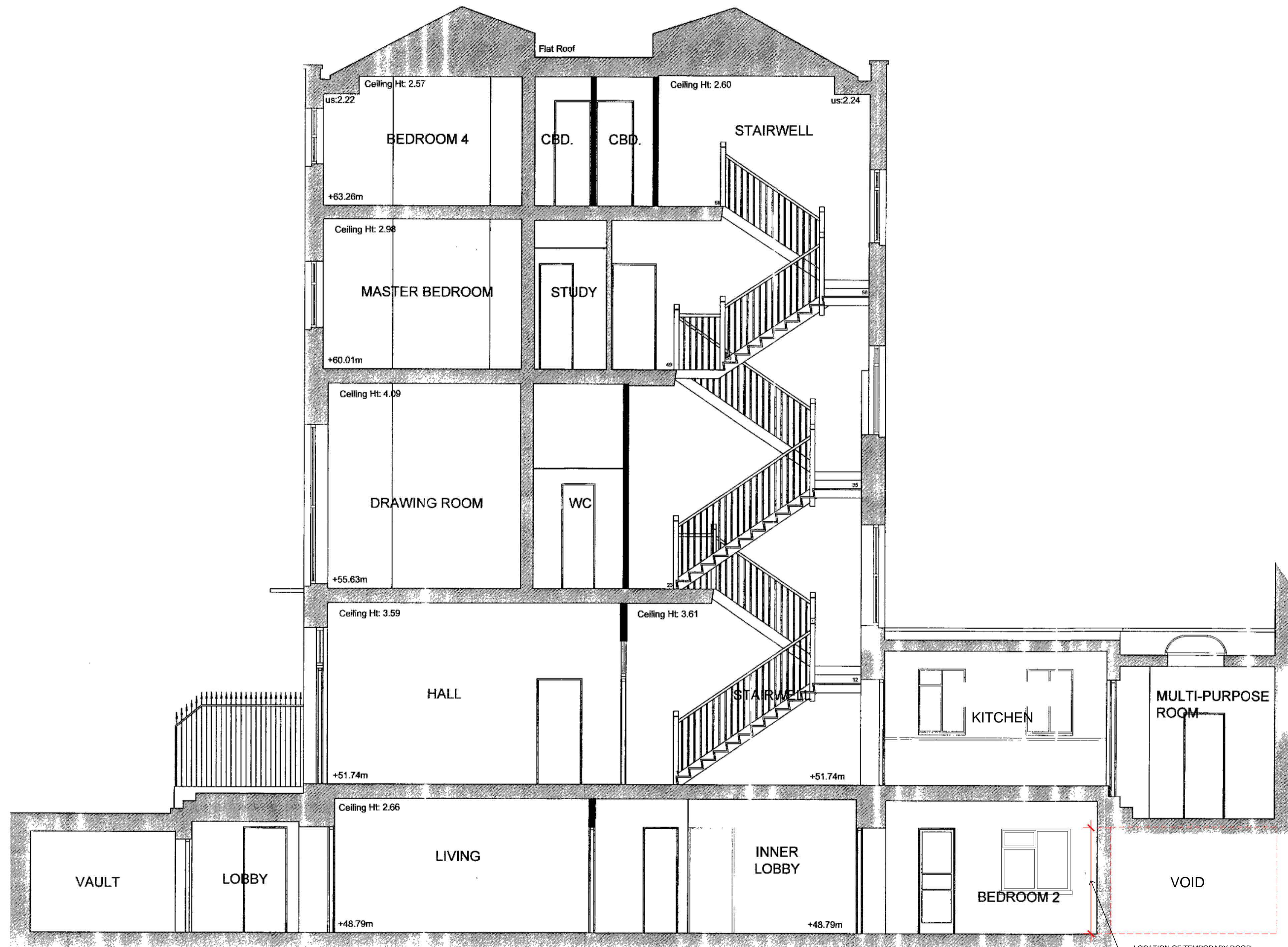
PROPOSED SECTION AA @1:50
