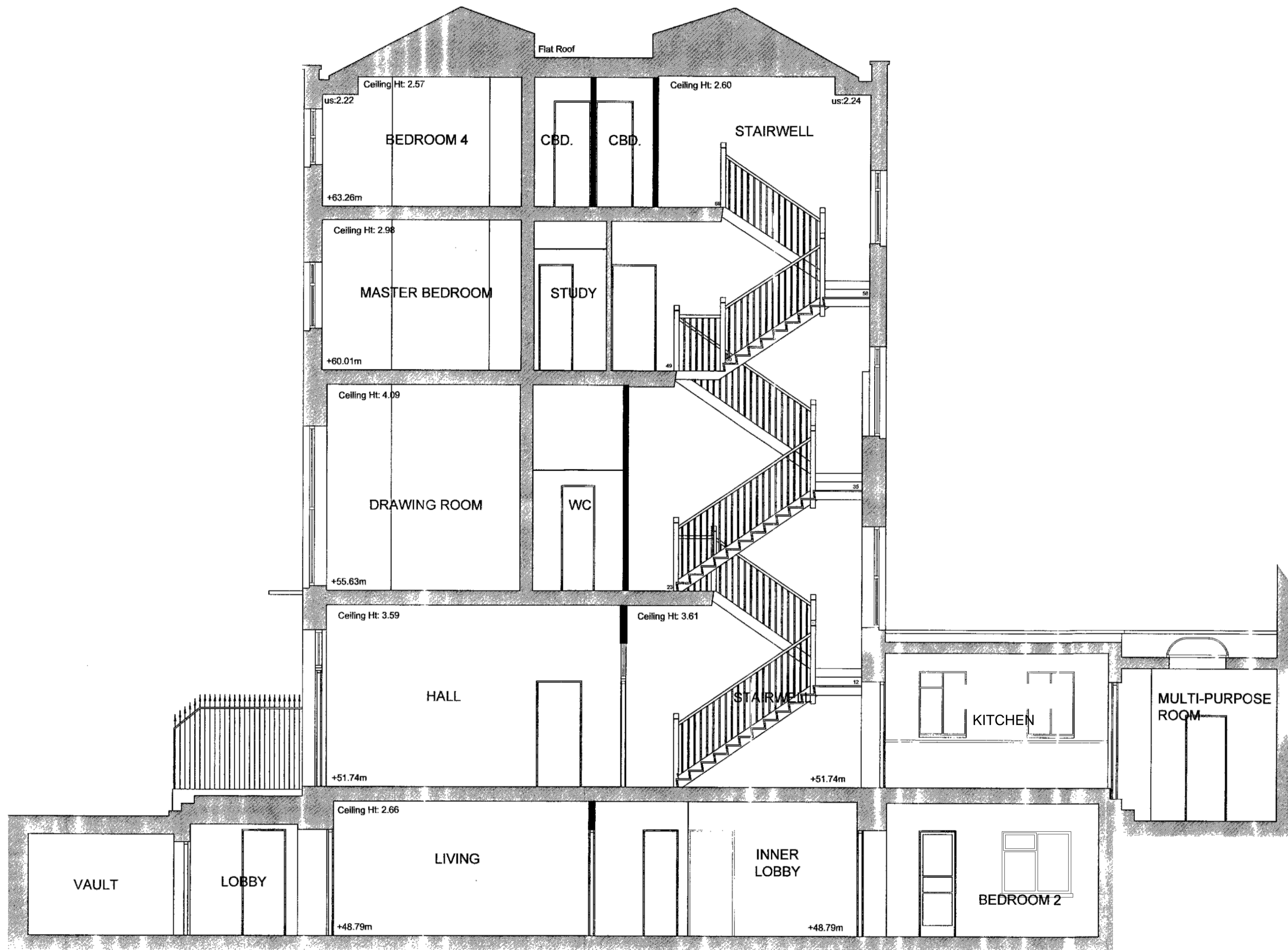
EXISTING SECTION AA @ 1:50
