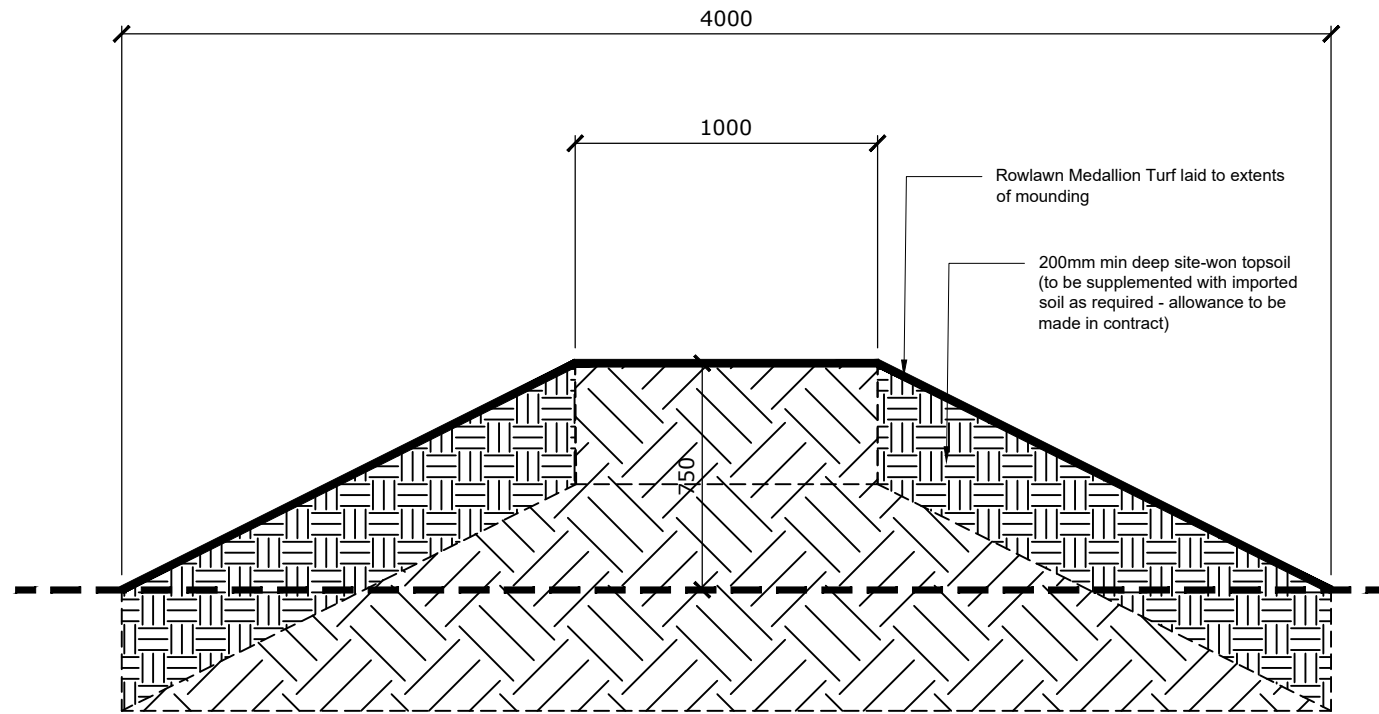
3 Grass mound Detail 1:25
