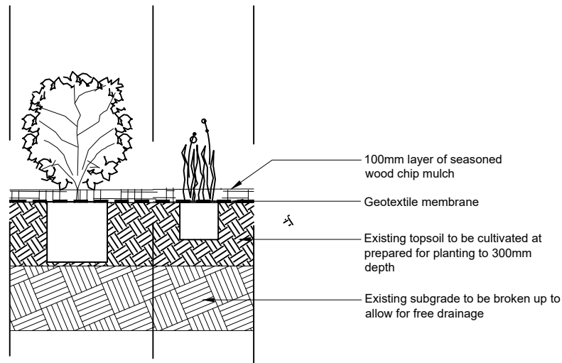
2 Shrub and Herbaceous Planting Detail 1:25
