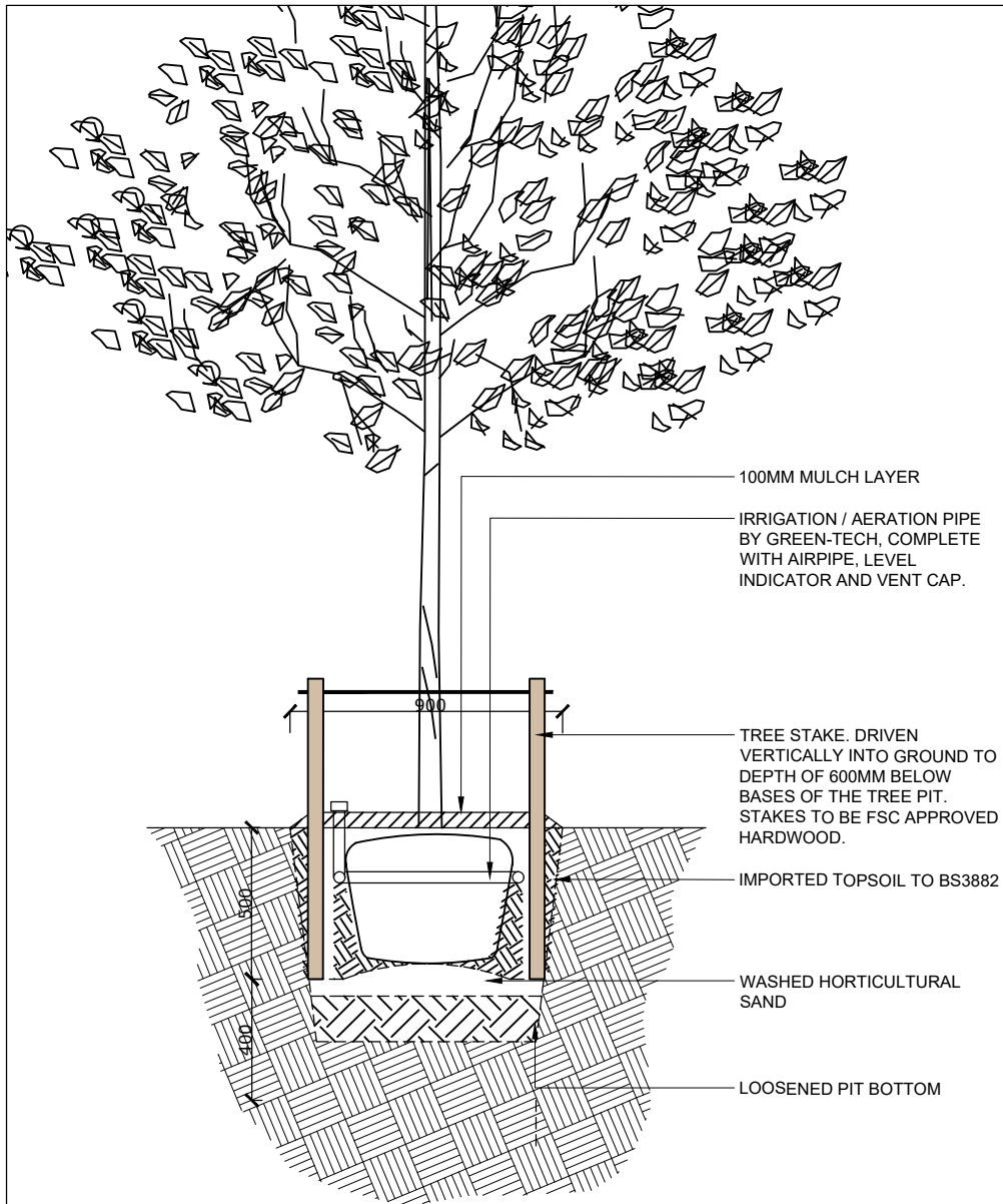
1 Tree Pit Detail 1:25
