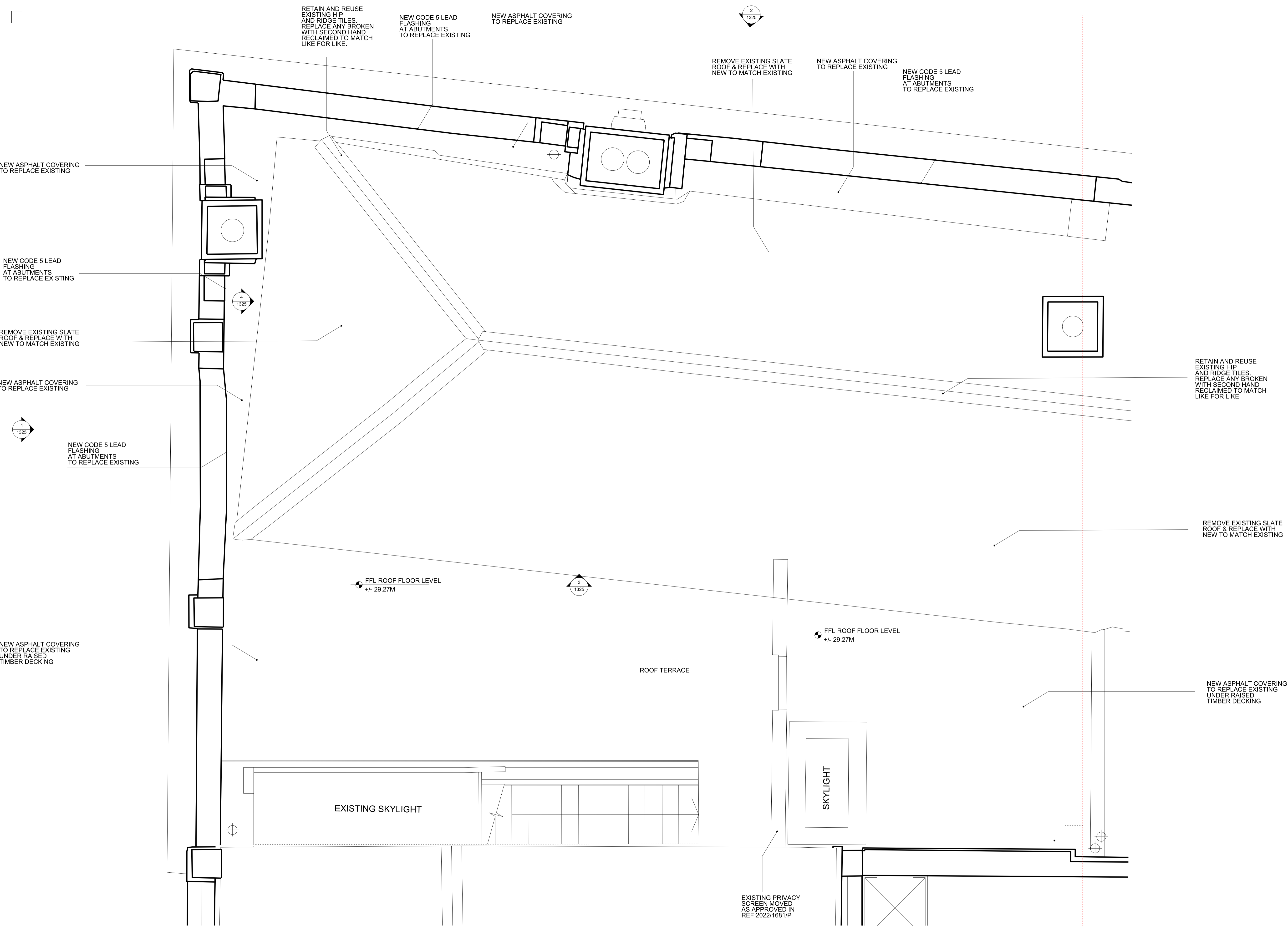
1 1:25 / 1:50 PROPOSED ROOF FINISHES PLAN
