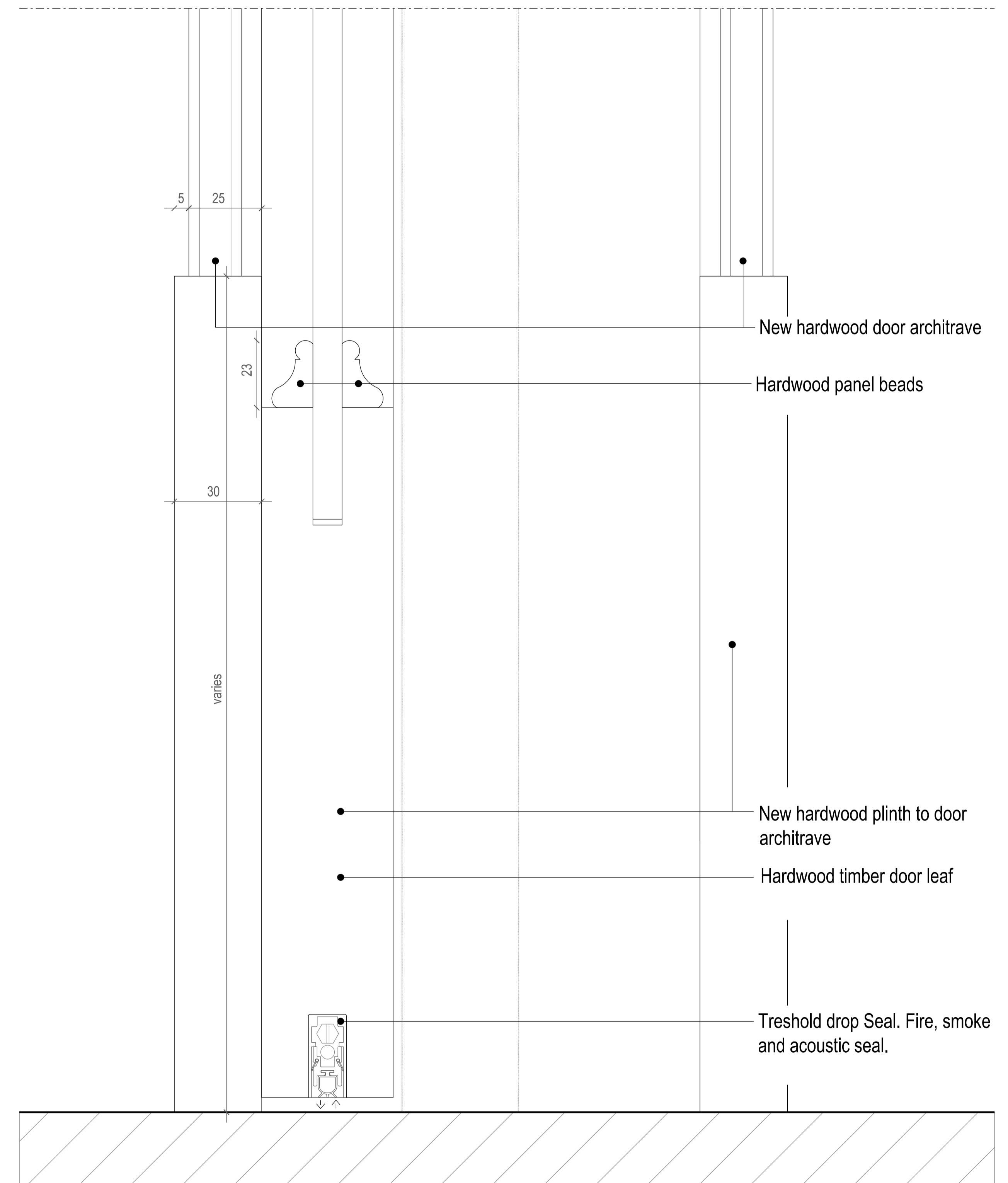
02 BASE OF DOOR DETAIL scale 1:1
