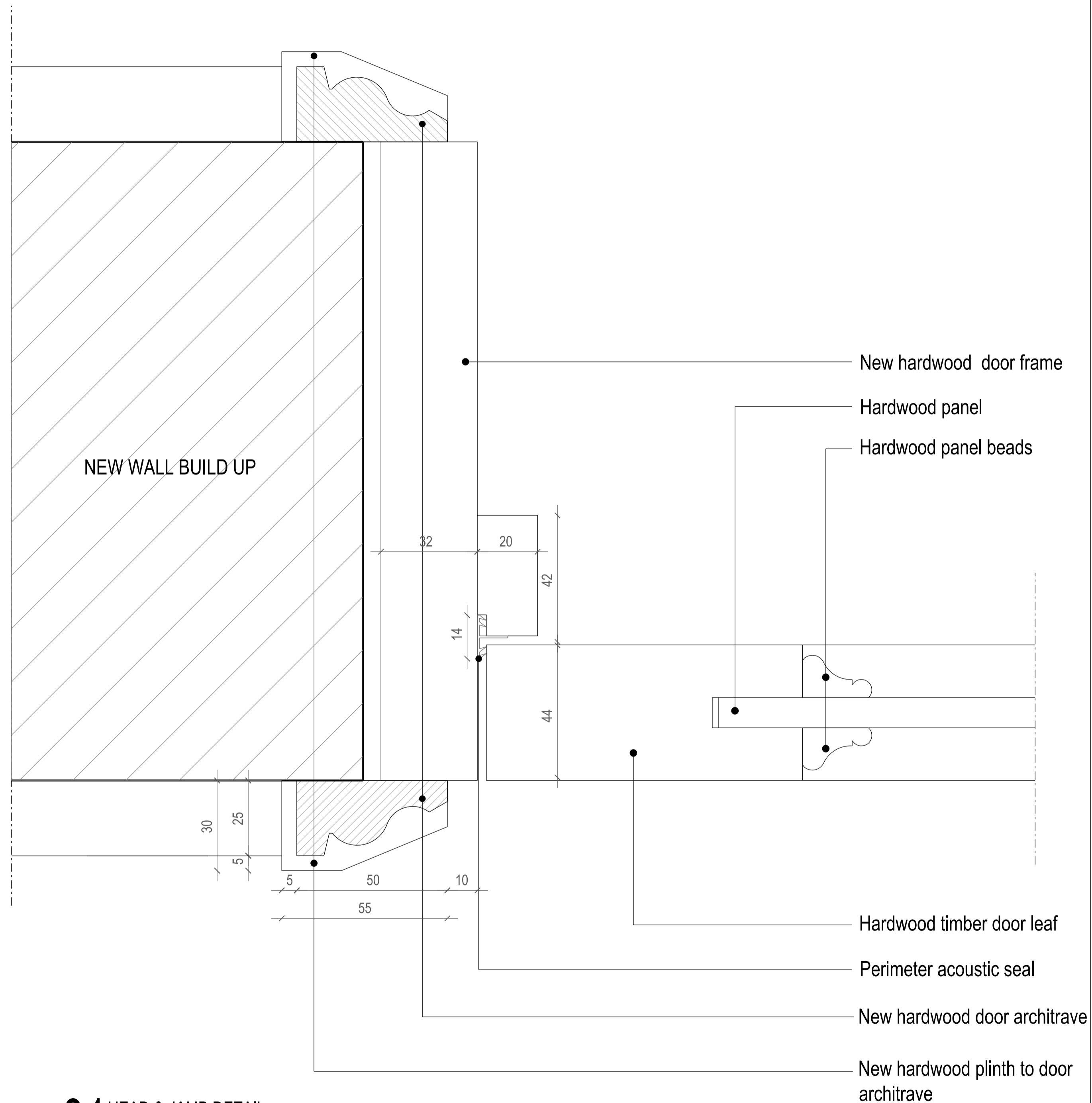
01 HEAD & JAMB DETAIL scale 1:1
