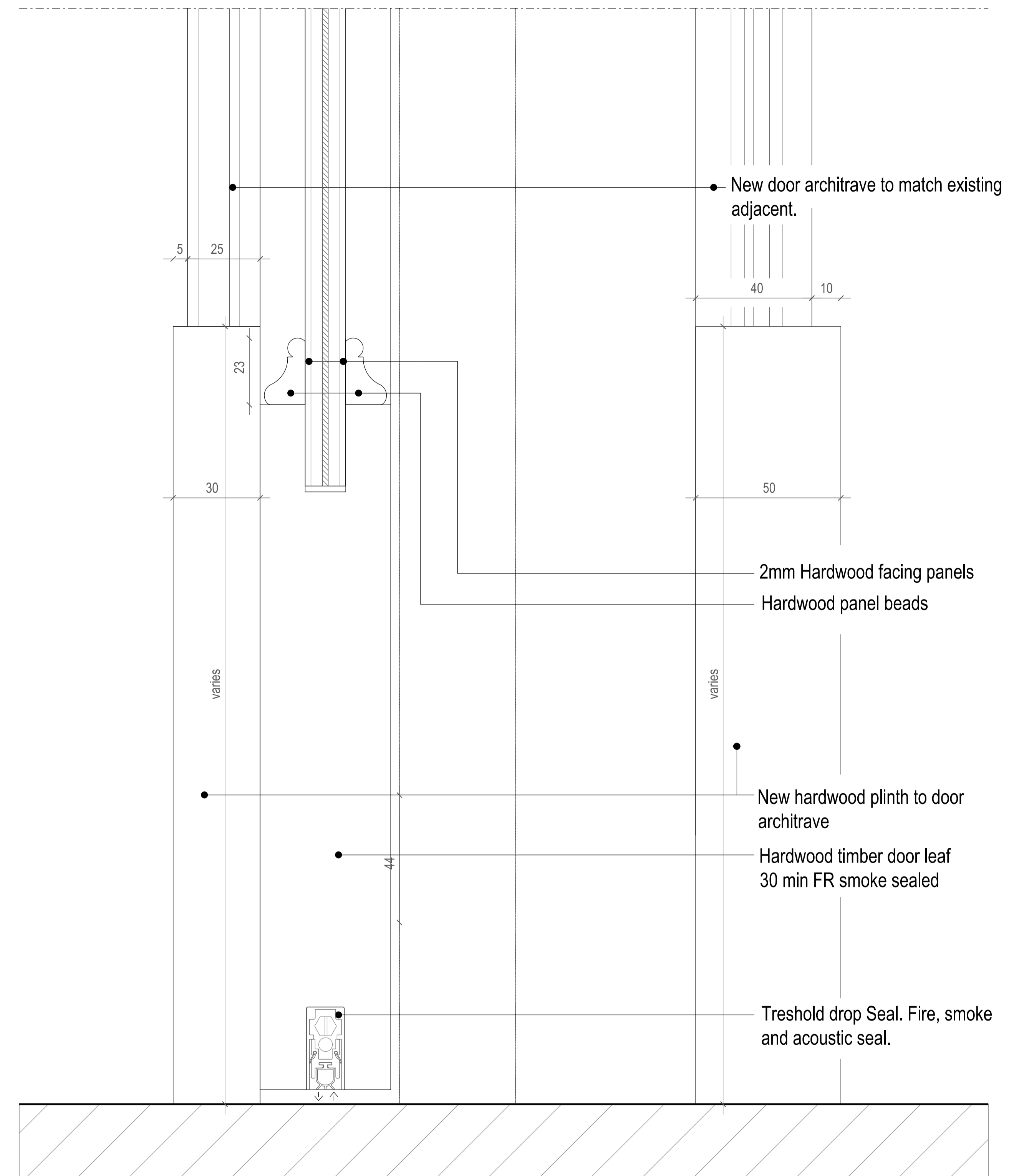
02 BASE OF DOOR DETAIL scale 1:1
