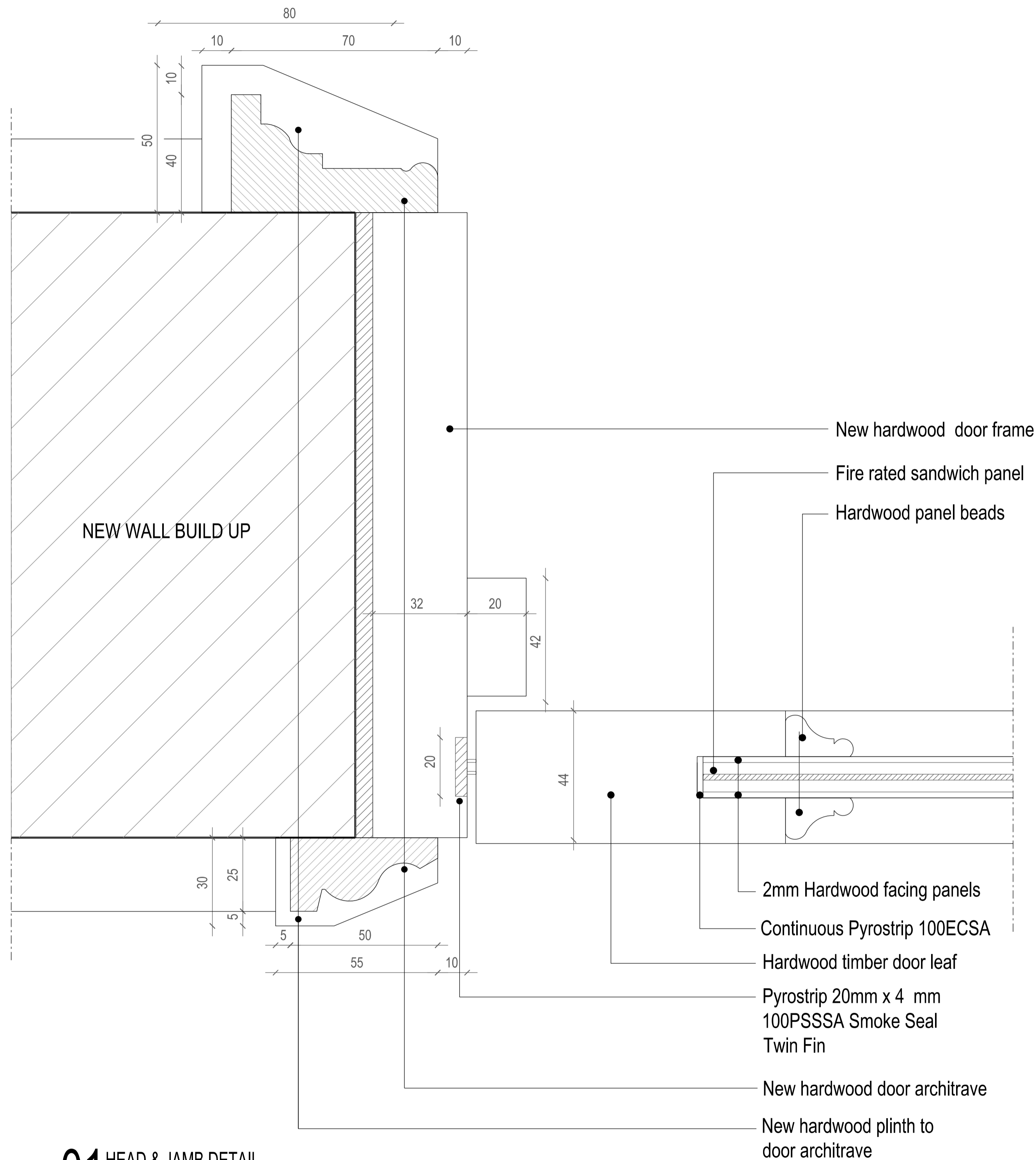
01 HEAD & JAMB DETAIL scale 1:1
