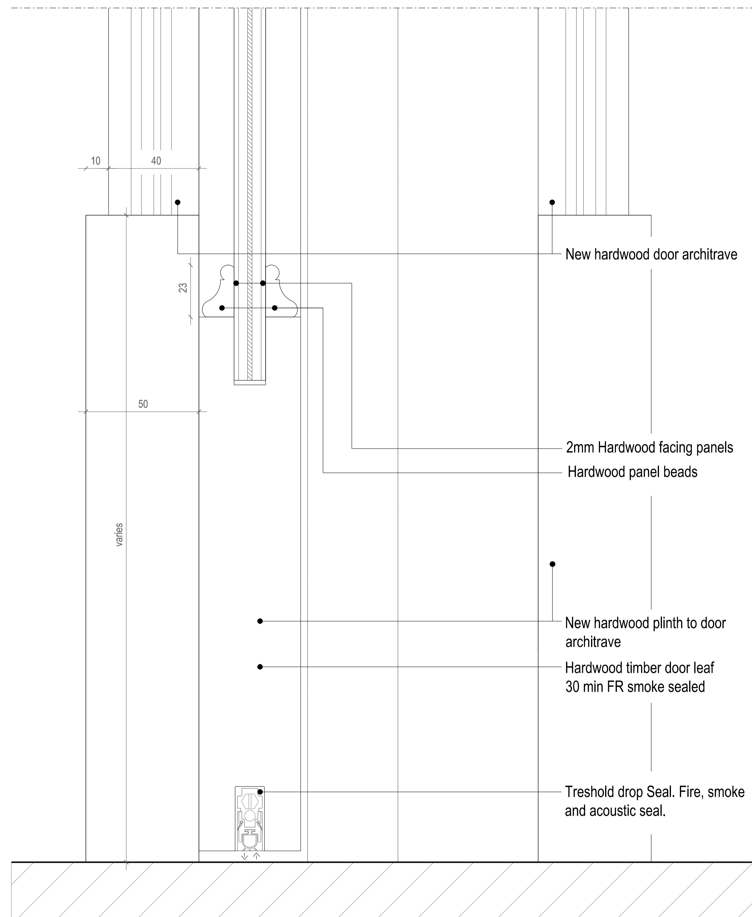
02 BASE OF DOOR DETAIL scale 1:1
