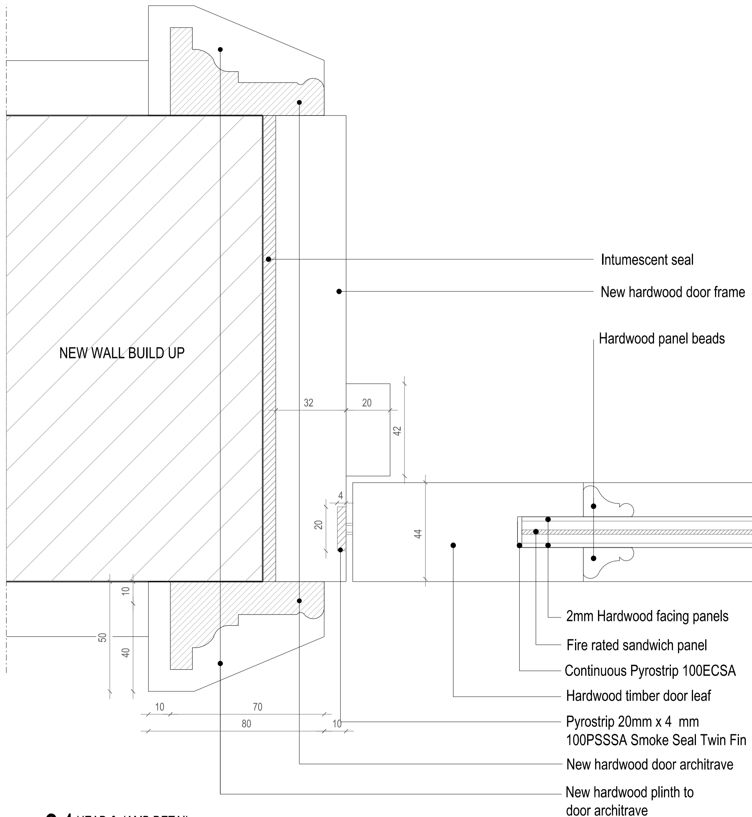
01 HEAD & JAMB DETAIL scale 1:1
