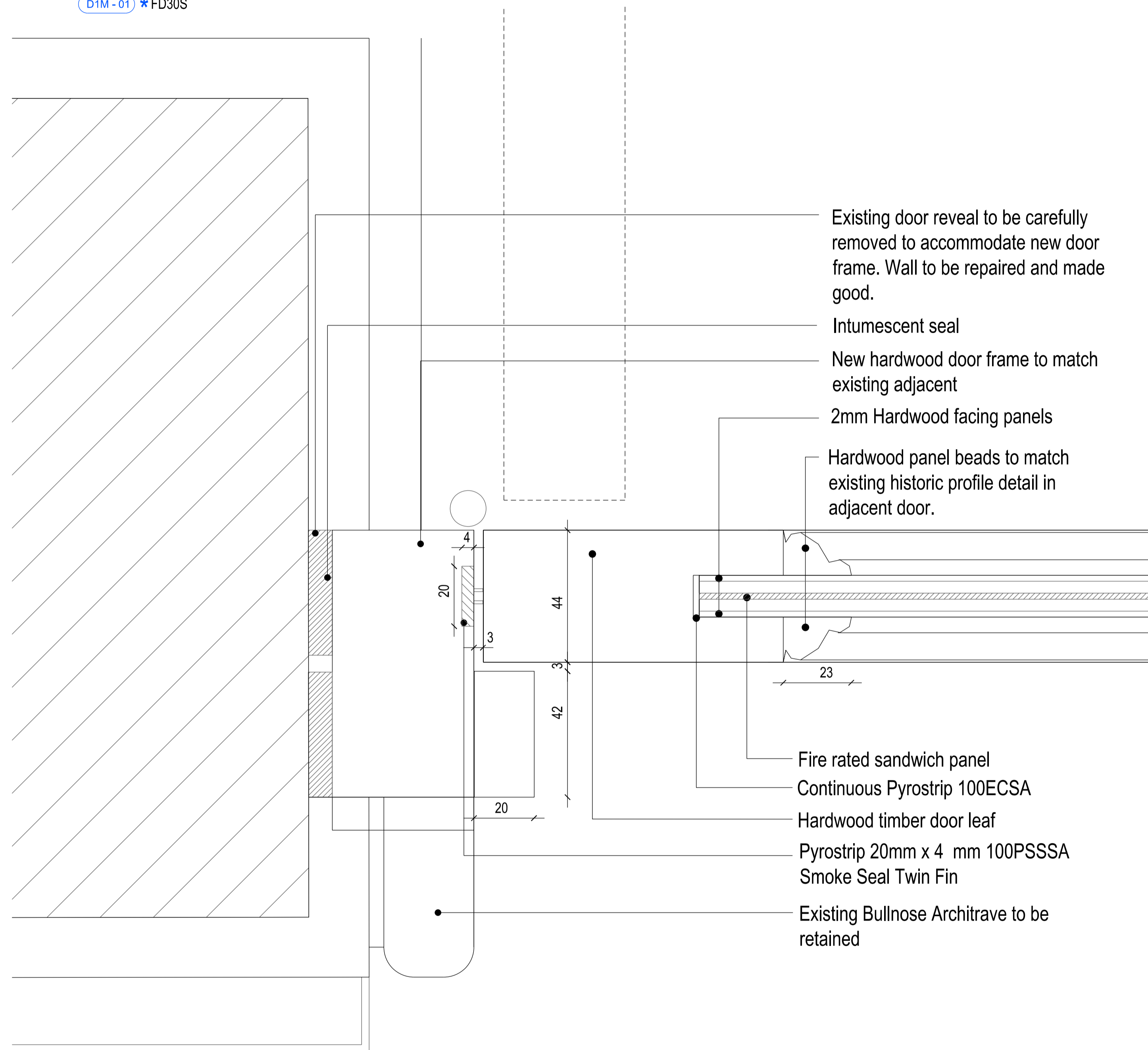
01 HEAD & JAMB DETAIL scale 1:1
