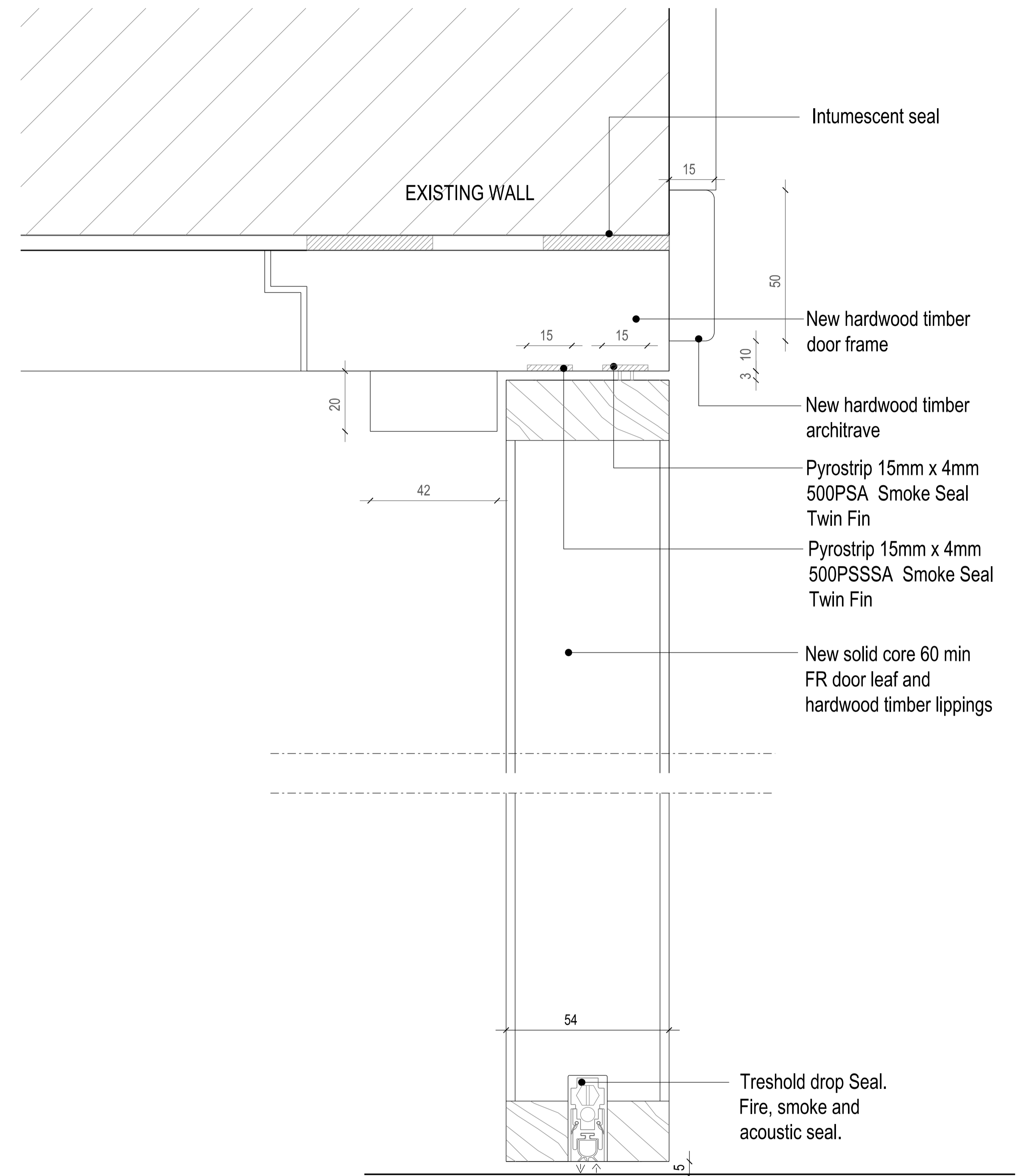
02 HEAD & BASE OF DOOR DETAIL scale 1:1
