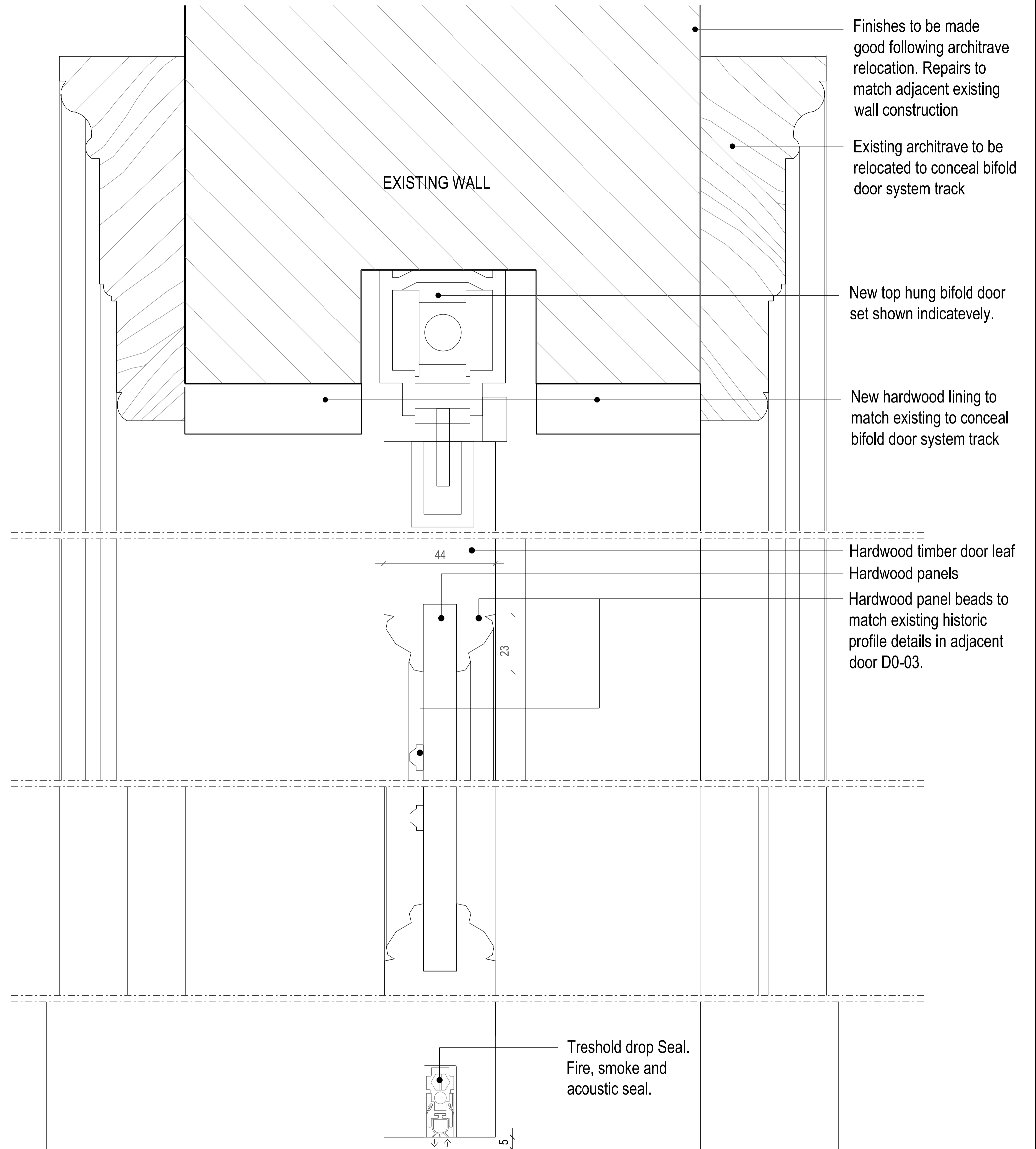
02 HEAD AND BASE OF DOOR DETAIL scale 1:1
