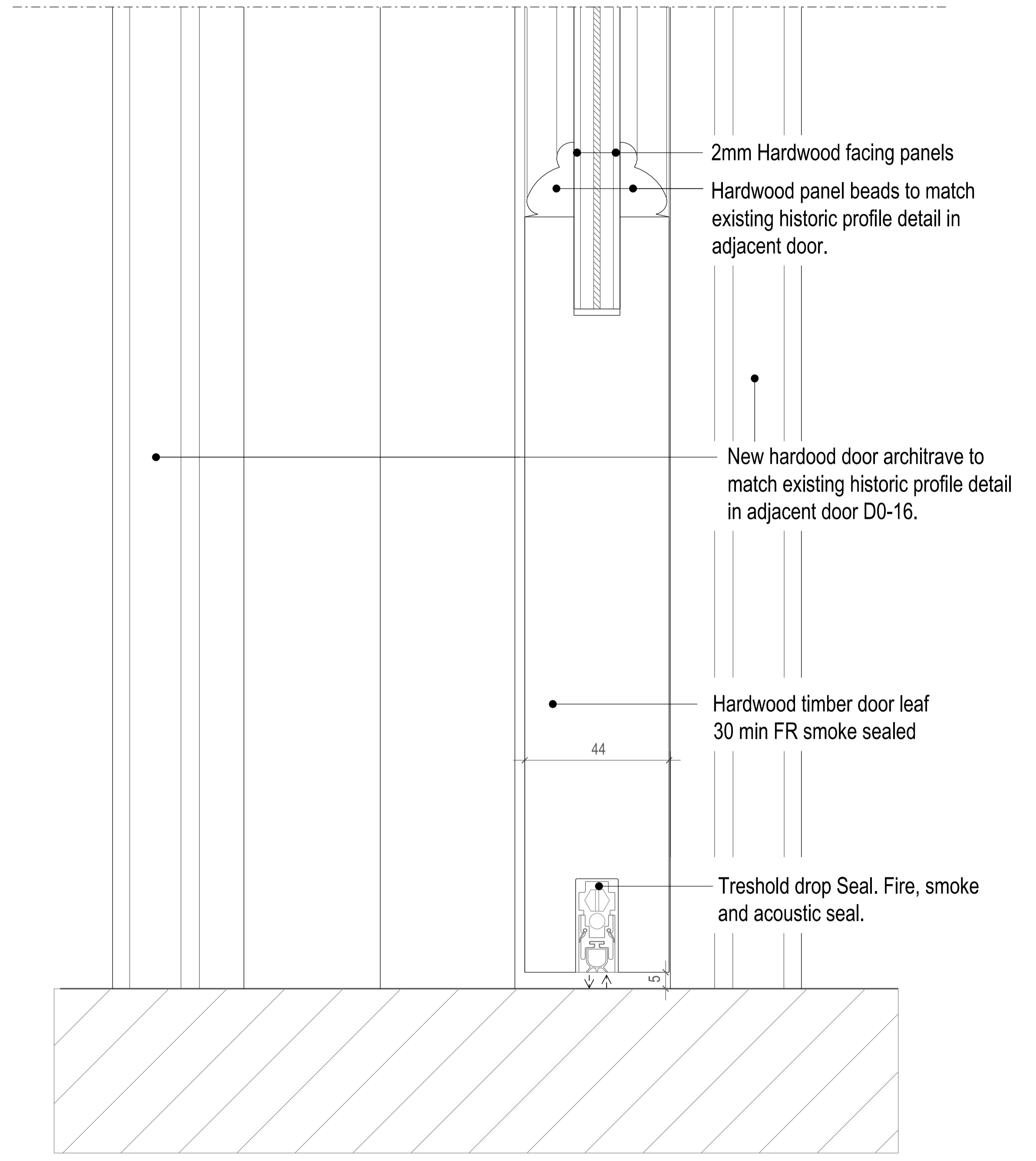
02 BASE OF DOOR DETAIL scale 1:1
