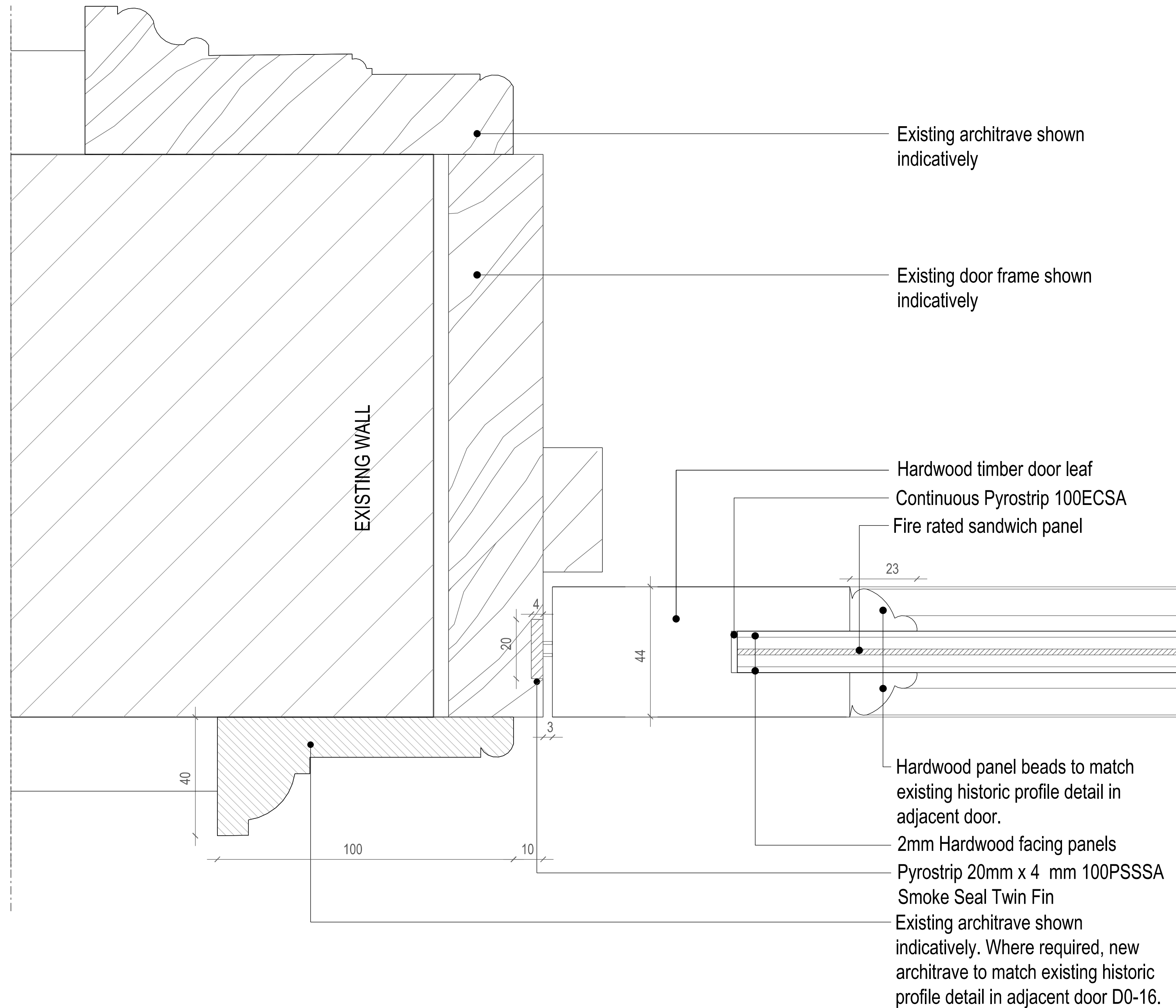
01 HEAD & JAMB DETAIL scale 1:1
